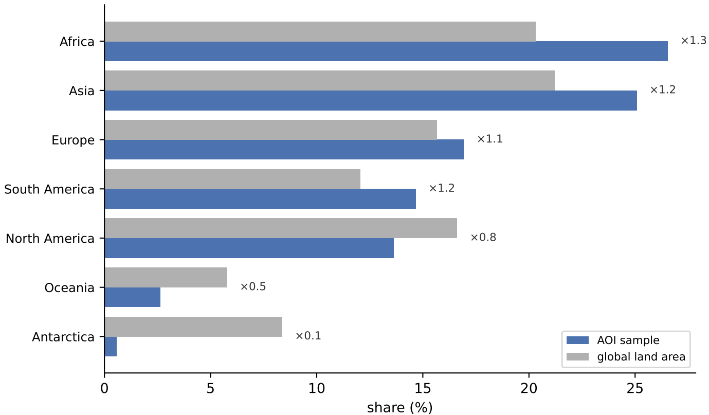
Continents: AOI sample vs global land area
