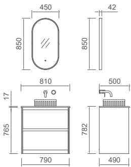
OJS274-800 Main Cabinet: 810x500x765mm Mirror: 450x42x850mm
