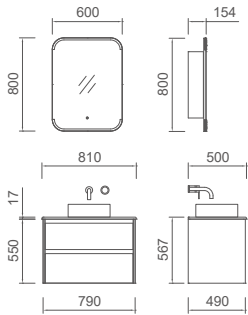
OJS275-800 Main Cabinet: 810x500x550mm Mirror: 600x154x800mm
