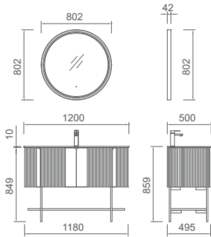
OJS246-1200 Main Cabinet: 1200x500x849mm Mirror: 802x42x802mm
