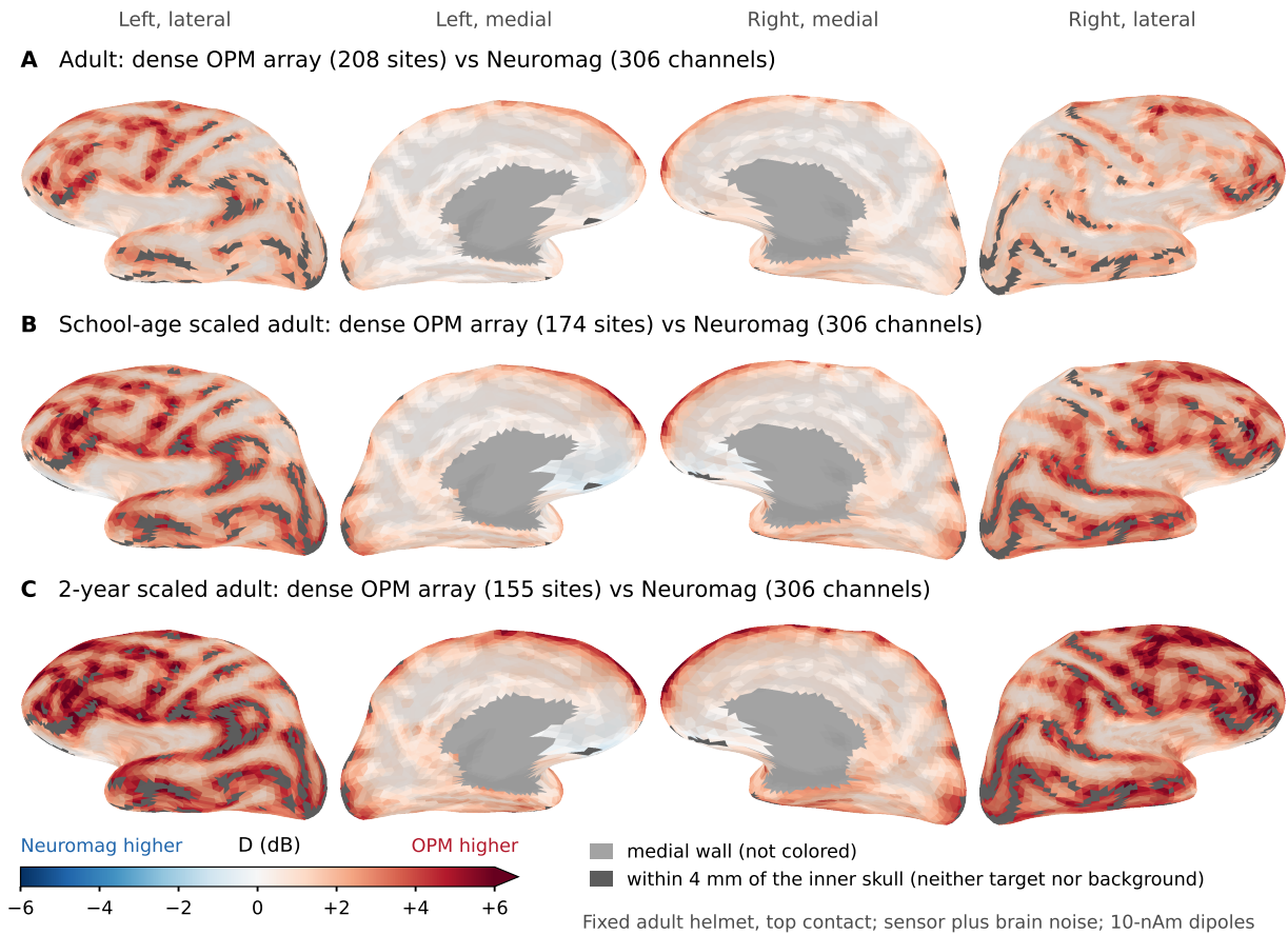
Fig. S10. Cortical maps of D in the adult and the scaled adults. Dense OPM array against Neuromag (306 channels), fixed adult helmet at top contact, sensor plus brain noise; inflated cortex, lateral and medial views of both hemispheres. (A) Adult (208 dense sites; area-weighted median D +1.00 dB). (B) School-age scaled adult (174 sites; +1.50 dB). (C) 2-year scaled adult (155 sites; +2.13 dB). The scaled adults share the adult's vertices. Red: the OPM's detectability is higher (color scale of main-text Fig. 6). Light gray: medial wall; dark gray: cortex within 4 mm of the inner skull, not simulated.
