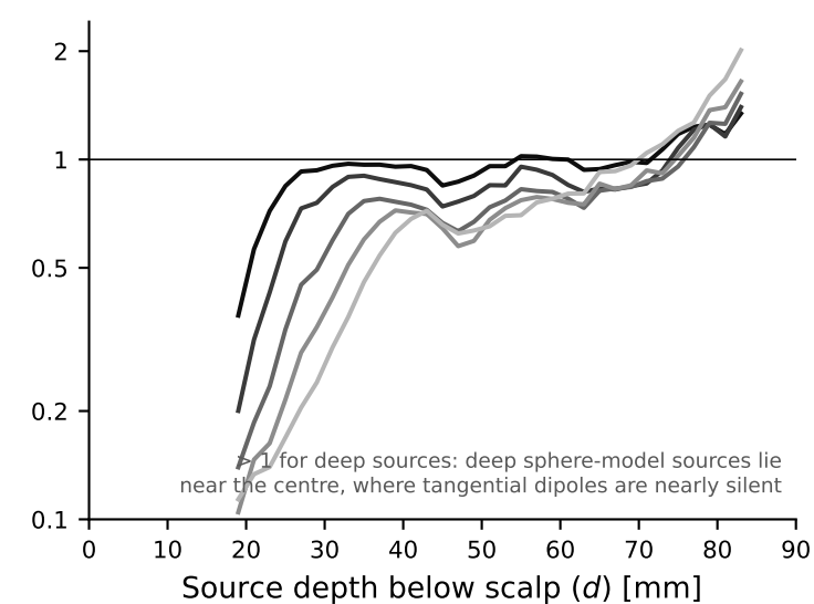
F OPM signal, realistic / sphere model (median)
