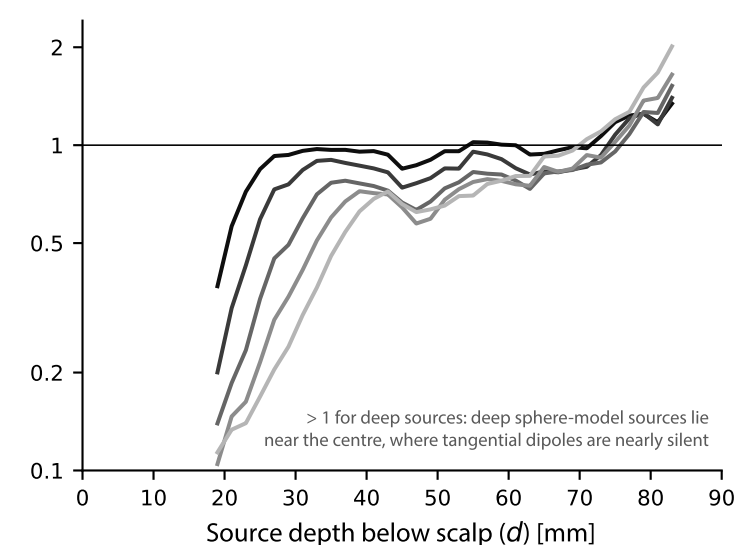
F OPM signal, realistic / sphere model (median)
