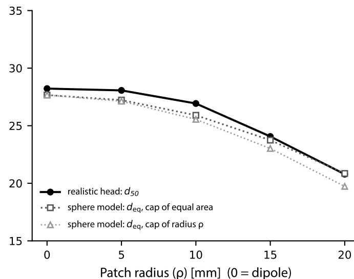
E Equal-SNR depth at \eta = 3 [mm]
