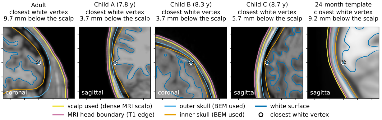
A Sections of 50 \times 50 mm through the white-surface vertex closest to the scalp used
