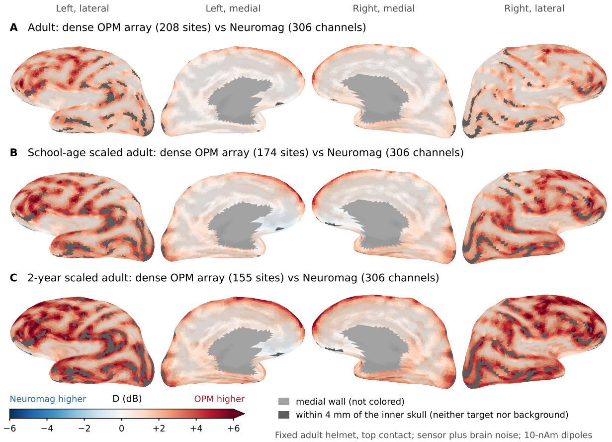
Fig. S10. Cortical maps of D in the adult and the scaled adults. Dense OPM array against Neuromag (306 channels), fixed adult helmet at top contact, sensor plus brain noise; inflated cortex, lateral and medial views of both hemispheres. (A) Adult (208 dense sites; area-weighted median D +1.00 dB). (B) School-age scaled adult (174 sites; +1.50 dB). (C) 2-year scaled adult (155 sites; +2.13 dB). The scaled adults share the adult's vertices. Red: the OPM's detectability is higher (color scale of main-text Fig. 6). Light gray: medial wall; dark gray: cortex within 4 mm of the inner skull, not simulated.
