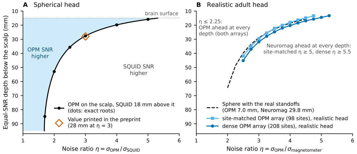
Fig. S1. The spherical benchmark and its transfer to a real head. (A) The spherical head of Jas et al. (2026), reimplemented: equal-SNR depth below the scalp against the noise ratio \eta = \sigma_{\text{OPM}} / \sigma_{\text{SQUID}} for a point magnetometer on the scalp (OPM) and one 18 mm above it (SQUID). Dots, exact roots at selected noise ratios; diamond, the preprint’s printed value (28 mm at \eta = 3 ); dotted line, the brain surface (15 mm below the scalp); shaded, the OPM’s single-channel SNR is higher. Adapted from Jas et al. (2026), Fig. 4E (CC BY 4.0, https://creativecommons.org/licenses/by/4.0/ ), redrawn from our reimplement of their model. (B) The same on the realistic adult head, with peak-channel SNR against the Neuromag magnetometers and sensor noise only, for the site-matched (98 sites, squares) and dense (208 sites, circles) arrays. Each array is drawn at the noise ratios at which it has a crossing; dashed, the sphere at the real median standoffs. SNR, signal-to-noise ratio; OPM, optically pumped magnetometer; SQUID, superconducting quantum interference device.
