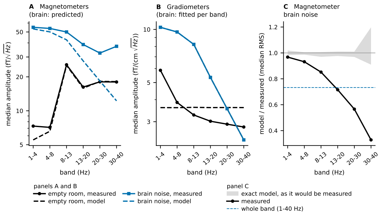
Fig. S4. The prediction by sub-band (1–4, 4–8, 8–13, 13–20, 20–30 and 30–40 Hz; background rescaled in each band on the gradiometers). (A) Magnetometers: median amplitude spectral density of the measured and modeled empty room (black) and brain noise (blue, the prediction). (B) Gradiometers: the measured brain noise and the model fitted to it per band (blue); the measured empty room and the model’s band-independent sensor noise (black). (C) The magnetometer brain-noise prediction per band, model over measured median RMS. Dashed, the whole-band value; gray, the exact-model range. RMS, root-mean-square.
