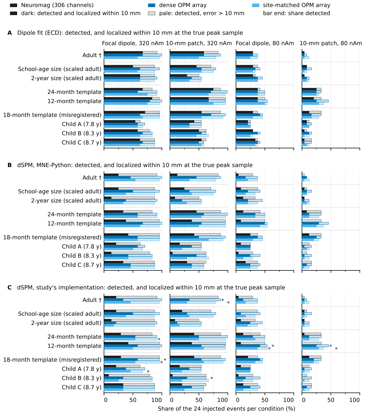
Fig. S15. Joint detection and localization, exploratory run. For each anatomy, system and condition (focal dipole or 10-mm patch at 320 and 80 nAm), the bar's end is the share of the 24 injected events detected by the practical detector. Its dark part is the share both detected and localized within 10 mm, its pale part the share detected but localized farther away. (A) Equivalent-current-dipole (ECD) fit. (B) dSPM through MNE-Python. (C) dSPM through the study's implementation. Stars: OPM minus Neuromag difference in joint success with p < 0.05 (exact McNemar, uncorrected; dipole fit and the study's dSPM only). The frozen thresholds gave 0.2–1.9 false events per minute on the localization study's held-out null data over the nine anatomies and three systems. Dagger: the adult at its measured head position; other heads at top contact. The heads reported separately (Section S10), the 18-month template (labeled misregistered) and children A–C, form the last block of rows. dSPM, dynamic statistical parametric mapping; OPM, optically pumped magnetometer.
