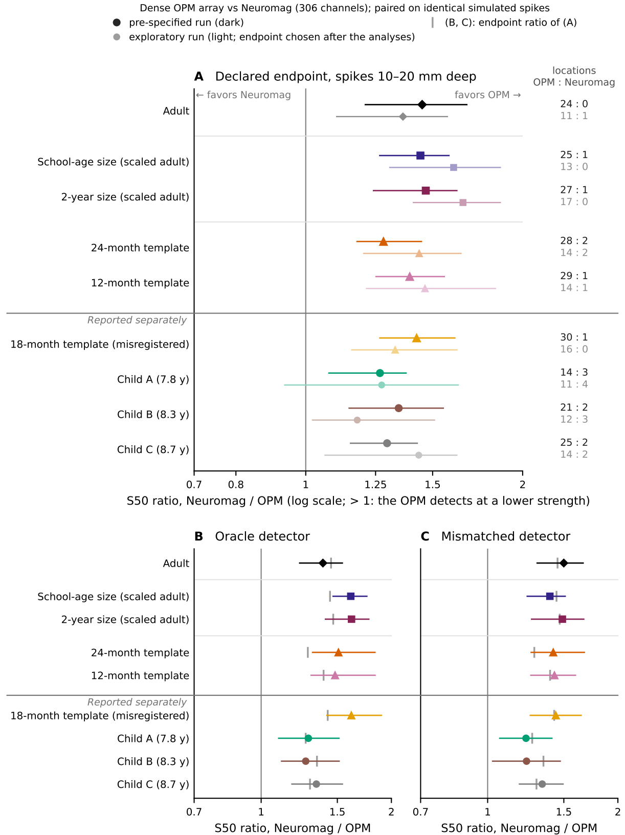
Fig. S18. Simulated interictal spikes, the pre-specified run, all nine anatomies. As main-text Fig. 10, with the 18-month template (triangles, labeled misregistered) and children A–C (circles) added below a divider labeled “Reported separately”. S50 ratio Neuromag/OPM for focal spikes 10–20 mm deep with (A) the practical detector, the declared endpoint (dark; light, the exploratory run), (B) the oracle detector and (C) the mismatched detector, with 95 % location-bootstrap intervals. Per-anatomy values and Holm-adjusted p values are in Table S11.
