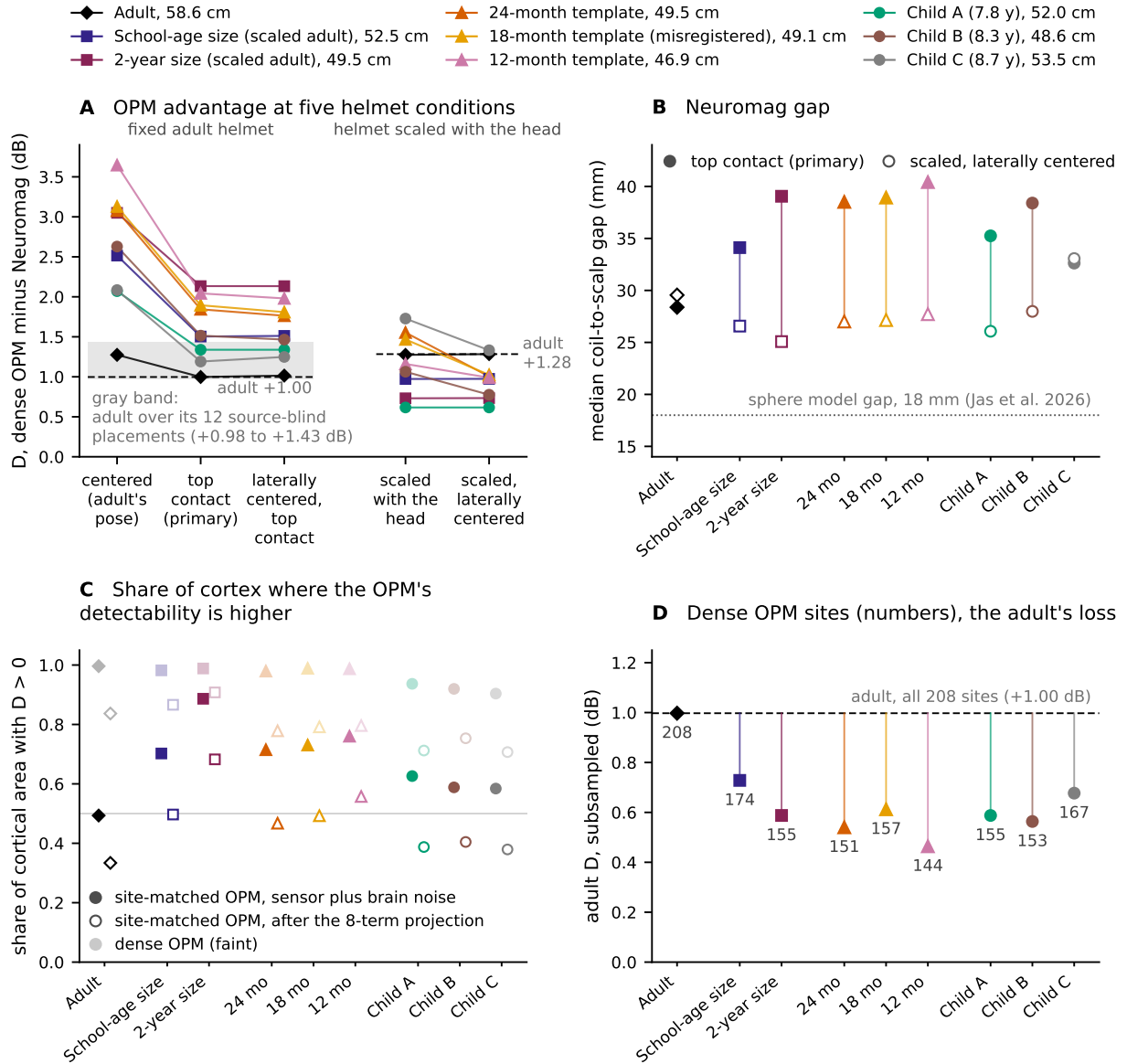
Fig. S8. The helmet scaled with the head and the routes of head size. Dense OPM array against Neuromag (306 channels), sensor plus brain noise; D , area-weighted median over cortical targets; heads ordered by class and head circumference, the children by label (A–C). (A) D under five helmet conditions: the fixed adult helmet at the centered pose, at top contact (primary) and laterally centered at top contact, and the helmet scaled with the head about the centered and the laterally centered head. Dashed lines: the adult at top contact and in its own scaled, laterally centered helmet (+1.28 dB); gray band: the adult over its 12 source-blind placements. (B) Median gap from magnetometer coil to scalp at top contact (filled) and in the scaled, laterally centered helmet (open); dotted: the 18-mm gap of the spherical benchmark (Jas et al., 2026). (C) Share of cortical area with D > 0 at top contact, site-matched array (filled: sensor plus brain noise; open: room field projected out) and dense array (faint). (D) Dense OPM sites per head (numbers) and the adult's D with its array subsampled to each count. Of the heads reported separately (Section S10), the 18-month template is labeled misregistered in the key, and the children are labeled A–C. The helmet fitted at the adult's gap is shown in main-text Fig. 9. OPM, optically pumped magnetometer.
