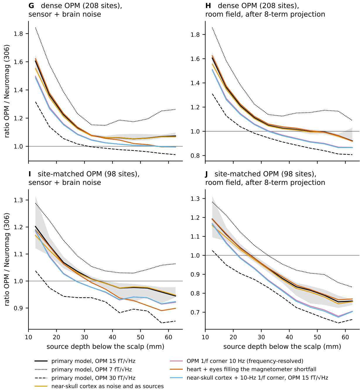
Fig. S5. (Continued.) (G–J) The ratio against depth below the scalp (5-mm bins) for the dense (G, H) and site-matched (I, J) arrays, with sensor plus brain noise (G, I) and projected (H, J). Black lines: the primary model at 15 fT/√Hz (with band), 7 fT/√Hz (dotted) and 30 fT/√Hz (dashed). Other lines: the near-skull cortex as noise and as sources; the 10-Hz corner under the frequency-resolved detector; the heart and eyes filling the magnetometer shortfall; and the near-skull cortex with the 10-Hz corner at 15 fT/√Hz.
