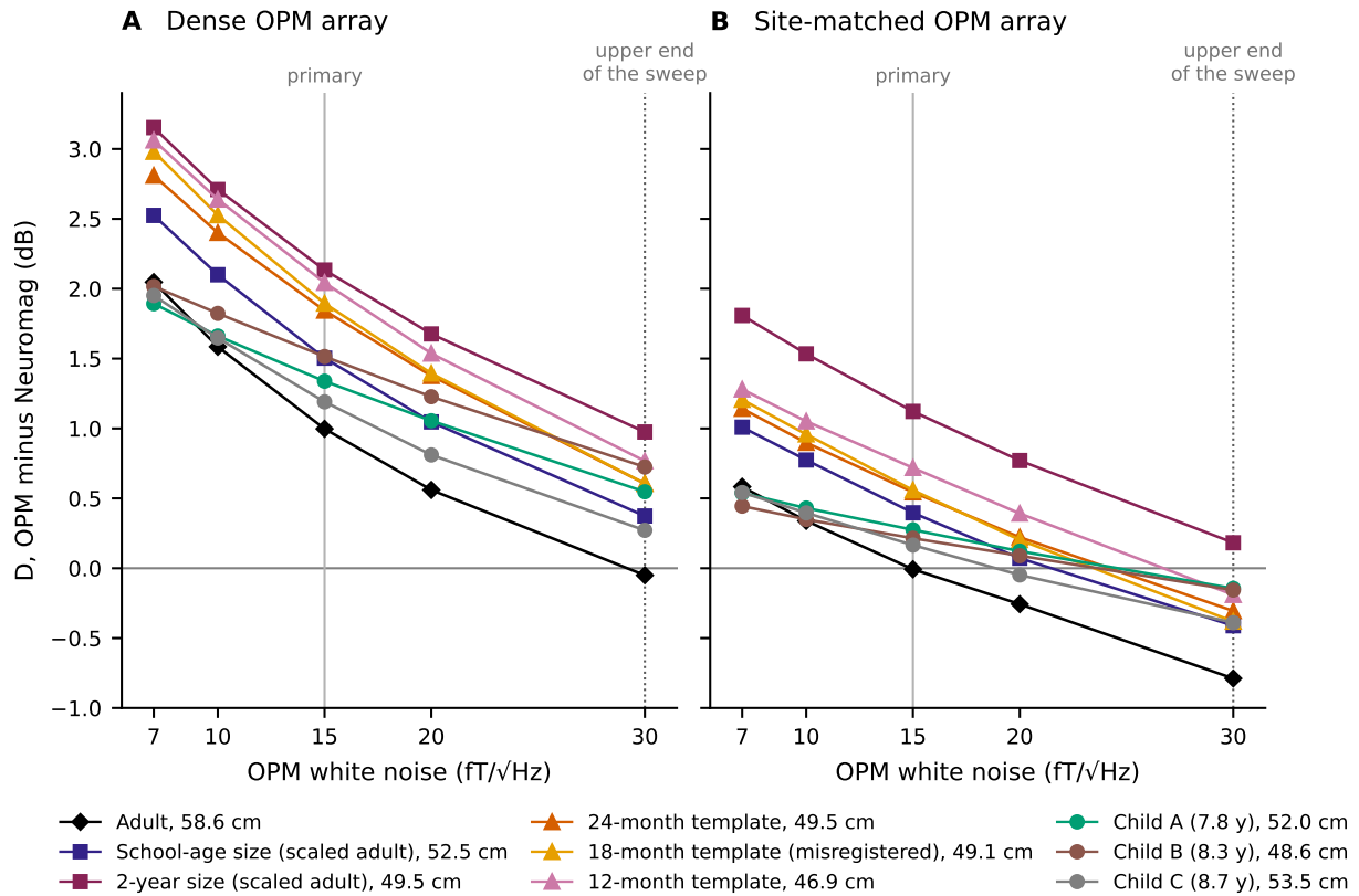
Fig. S11. The OPM noise level across heads. D (fixed adult helmet at top contact) against the OPM's white sensor noise (7, 10, 15, 20 and 30 fT/√Hz), Neuromag's noise unchanged, for the adult and the eight smaller heads. (A) Dense OPM array. (B) Site-matched OPM array. Solid vertical line: the primary 15 fT/√Hz; dotted line: 30 fT/√Hz, the upper end of the sweep, near the empty-room OPM floor of Jas et al. (2026) (Section S8.3). Points: medians, without intervals. Of the heads reported separately (Section S10), the 18-month template is labeled misregistered in the key, and the children are labeled A–C.
