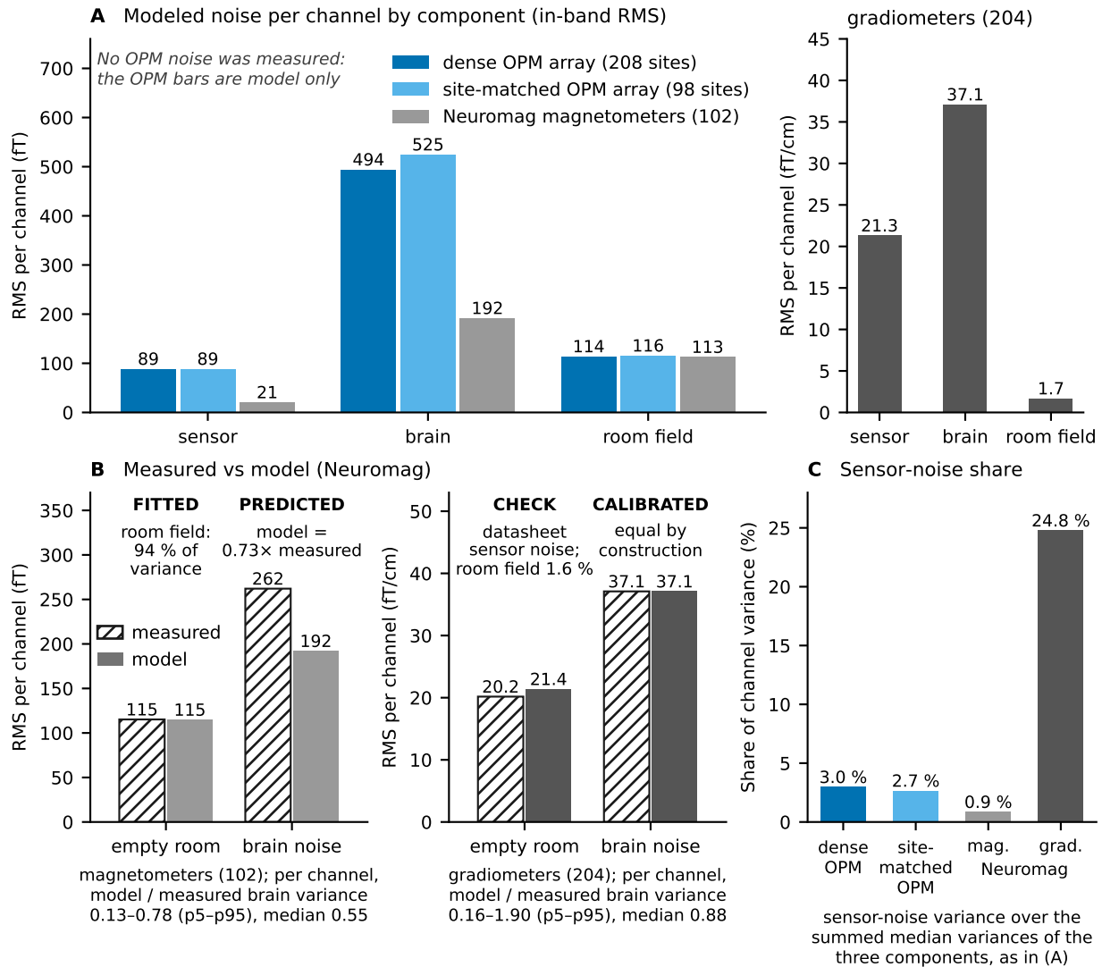
Fig. S2. The noise budget and what is fitted, checked, calibrated and predicted. (A) Modeled in-band RMS noise per channel by component (sensor noise, cortical background, room field): the square root of each component's median channel variance (RMS values do not add). Shown are the dense OPM array (208 sites), the site-matched OPM array (98 sites) and Neuromag's 102 magnetometers, and the 204 gradiometers on their own fT/cm axis. The OPM bars are model only. (B) Measured Neuromag quantities against the model: the empty-room level (magnetometers, a fit; gradiometers, a check) and the brain noise (magnetometers, a prediction; gradiometers, calibrated). Labels under the panels give the median and the 5th to 95th percentiles over channels of the modeled-to-measured brain-noise variance. The covariance check of Section S3.4 excludes the bad channel, so its gradiometer range differs slightly. (C) The sensor-noise share of the in-band variance with brain noise and room field. RMS, root-mean-square.
