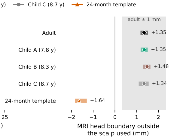
Fig. S6. MRI quality check of the school-aged children, with the adult and the 24-month template as references; surfaces as the forward models use them. (A) Sections of 50 × 50 mm through the white-surface vertex closest to the scalp used (open circle), sagittal or coronal, whichever contains more of the scalp's outward normal there. Gray: T1 intensity; yellow: dense MRI scalp used; pink: MRI head boundary (Otsu level along the scalp normals); light blue and orange: outer and inner skull of the BEM used (modeled in the children; Section S4.1); dark blue: white surface. (B) Cumulative share of white-surface vertices against distance to the scalp used (solid) and to the MRI head boundary (dashed), lowest quarter; dotted: the 8 and 10-mm threshold. (C) Offset of the MRI head boundary from the scalp used above the fiducial plane, positive outward: median and quartiles; shaded: the adult's median ± 1 mm, the verdict's tolerance. Children: OpenNeuro ds005234 (Fadeev et al., 2024, 2025); template: O'Reilly et al. (2021); adult: MNE sample data. BEM, boundary-element model.
