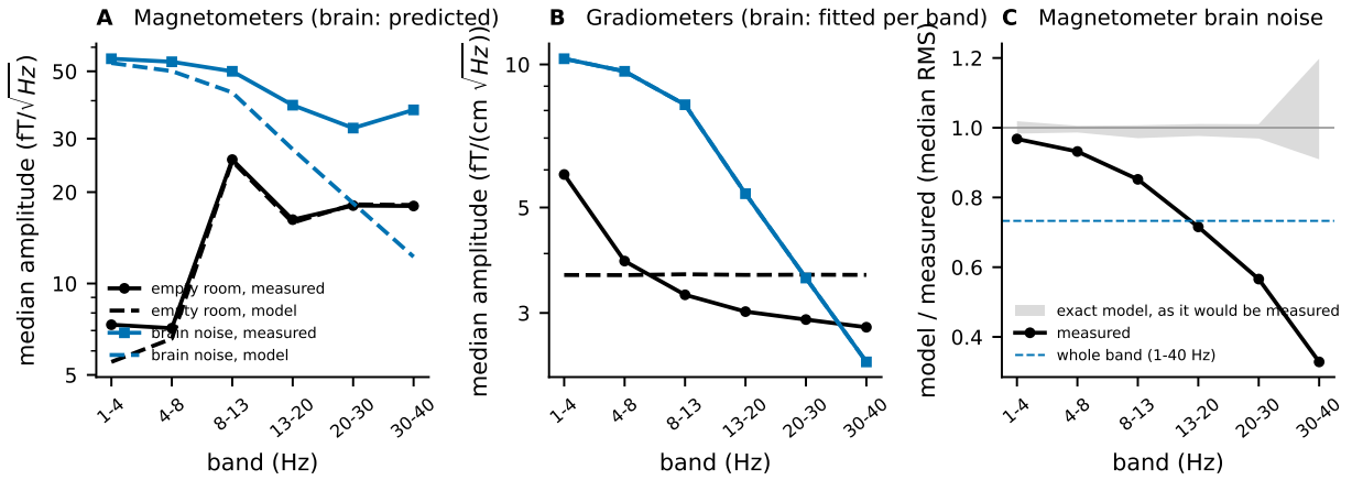
Fig. S4. The prediction by sub-band (1–4, 4–8, 8–13, 13–20, 20–30 and 30–40 Hz; background rescaled in each band on the gradiometers). (A) Magnetometers: median amplitude spectral density of the measured and modeled empty room (black) and brain noise (blue, the prediction). (B) Gradiometers: the measured brain noise and the model fitted to it per band (blue); the measured empty room and the model’s band-independent sensor noise (black). (C) The magnetometer brain-noise prediction per band, model over measured median RMS. Dashed, the whole-band value; gray, the exact-model range. RMS, root-mean-square.
