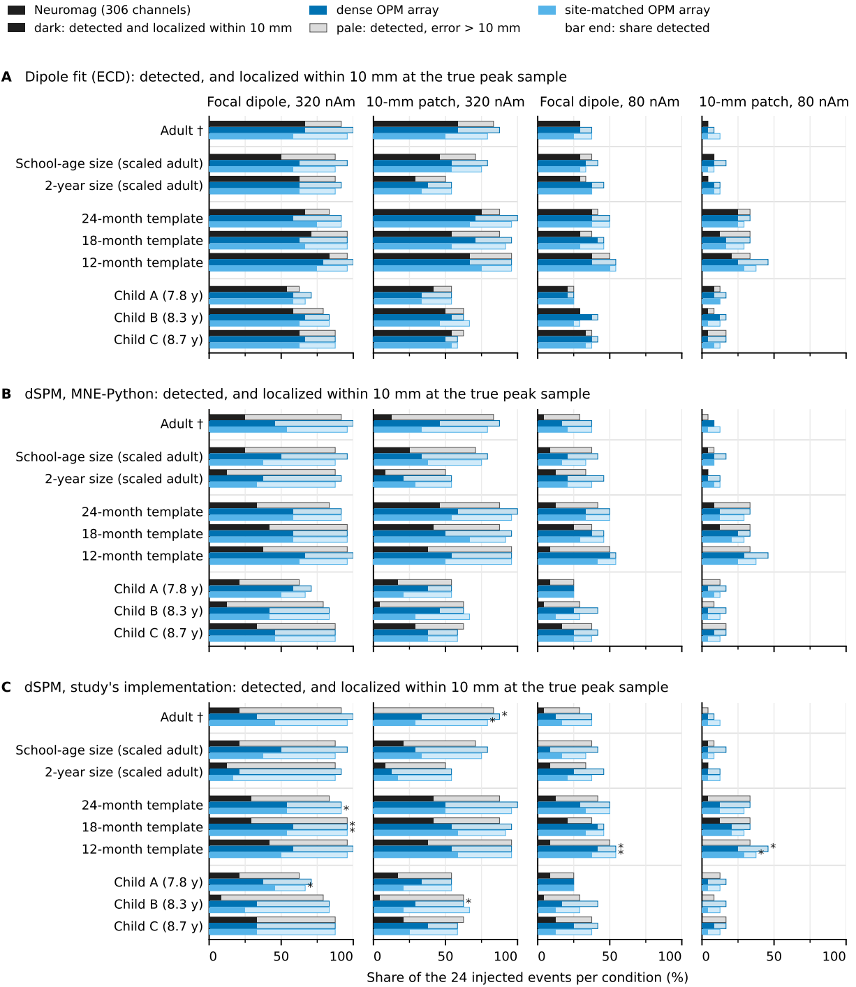
Fig. S15. Joint detection and localization, exploratory run. For each anatomy, system and condition (focal dipole or 10-mm patch at 320 and 80 nAm), the bar's end is the share of the 24 injected events detected by the practical detector; its dark part is the share both detected and localized within 10 mm, its pale part the share detected but localized farther away. (A) Equivalent-current-dipole (ECD) fit. (B) dSPM through MNE-Python. (C) dSPM through the study's implementation. Stars: OPM minus Neuromag difference in joint success with p < 0.05 (exact McNemar, uncorrected; dipole fit and the study's dSPM only). The frozen thresholds gave 0.2–1.9 false events per minute on the localization study's held-out null data over the nine anatomies and three systems. Dagger: the adult at its measured head position; other heads at top contact. dSPM, dynamic statistical parametric mapping; OPM, optically pumped magnetometer.
