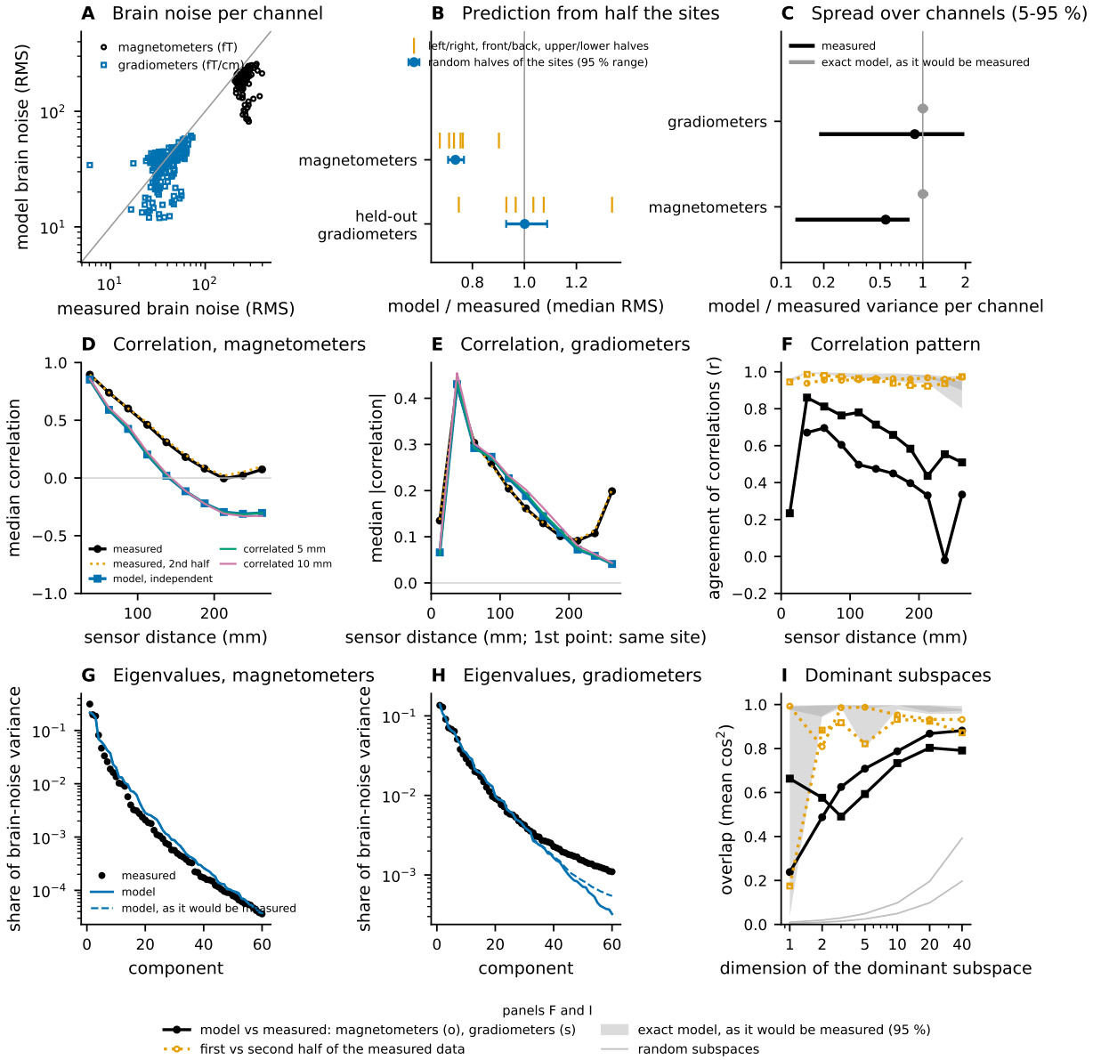
Fig. S3. Structure of the measured and modeled Neuromag brain noise (task baseline minus empty room, 1–40 Hz). (A) Modeled against measured RMS brain noise per channel (magnetometers, fT; gradiometers, fT/cm; logarithmic axes; diagonal, equality). (B) Model over measured median amplitude, scale fitted on half the sites: random halves (1,000 splits; dot and 95 % range) and six directional halves (ticks: left and right, front and back, upper and lower), for the magnetometers and the held-out gradiometers. (C) The 5th to 95th percentile over channels of the modeled-to-measured variance (black) and the exact-model range (gray). (D) Median correlation between magnetometers against distance: measured (both halves of the recording), the model with independent background sources and with correlation lengths of 5 and 10 mm. (E) The same for the gradiometers as the median absolute correlation; the first point is the two gradiometers of one site. (F) Agreement of the correlation patterns per distance bin (Pearson r over channel pairs): model against measurement (black; circles, magnetometers; squares, gradiometers), the two halves of the measurement (orange, dotted) and the exact-model band (gray). (G, H) Eigenvalue spectra as shares of the variance: measured (dots), model (line) and model as measured (dashed). (I) Overlap (mean squared cosine) of the dominant subspaces of model and measurement against subspace dimension, with the two halves of the measurement (orange), the exact-model band (gray) and random subspaces (thin gray lines). Exact-model ranges and bands come from surrogates measured like the recording. RMS, root-mean-square.
