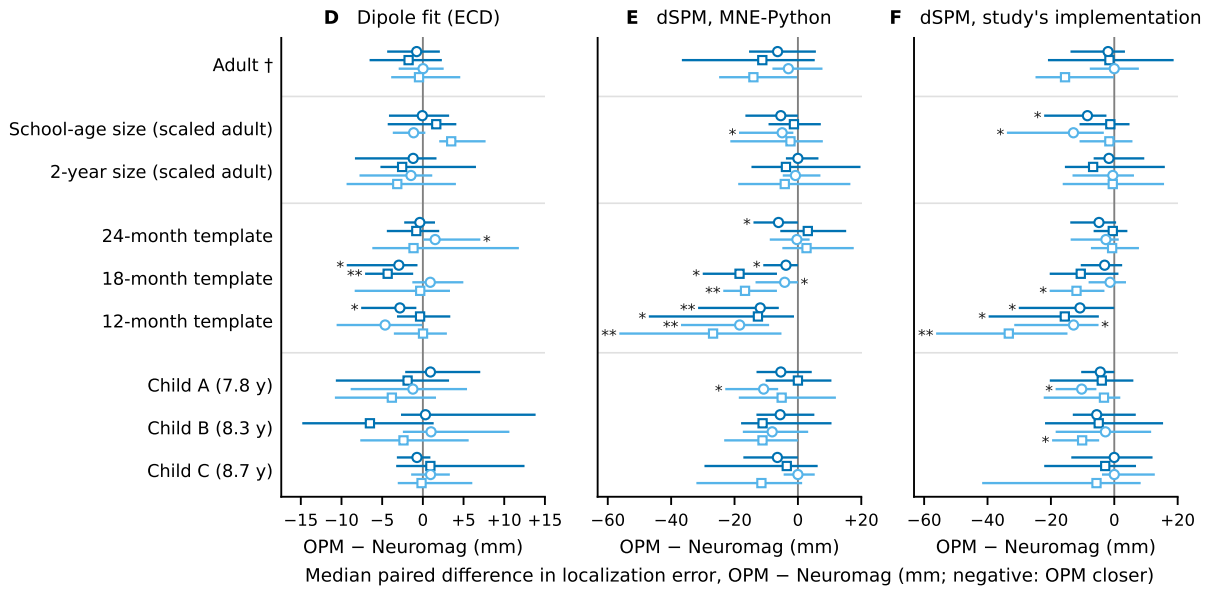
Fig. S14. Localization effect sizes, exploratory run. Median over the 24 events of a condition of the paired difference in localization error, OPM array minus Neuromag (306 channels), with 95 % bootstrap intervals over events (2,000 resamples); negative: the OPM array localizes closer to the true source. (A, D) Equivalent-current-dipole (ECD) fit. (B, E) dSPM through MNE-Python. (C, F) dSPM through the study's implementation. (A–C) 320 nAm. (D–F) 80 nAm, where the errors are mostly those of undetected events. Colors and marker shapes as in the key; filled markers: both systems detected at least half of the events (practical detector); open markers: fewer. Stars: uncorrected Wilcoxon signed-rank p < 0.05 (one) and p < 0.0025 , the Bonferroni threshold over the 20 comparisons of one anatomy and OPM array (two). The x axes differ between strengths and between the dipole and dSPM columns. Dagger: the adult at its measured head position; other heads at top contact. dSPM, dynamic statistical parametric mapping; OPM, optically pumped magnetometer.
