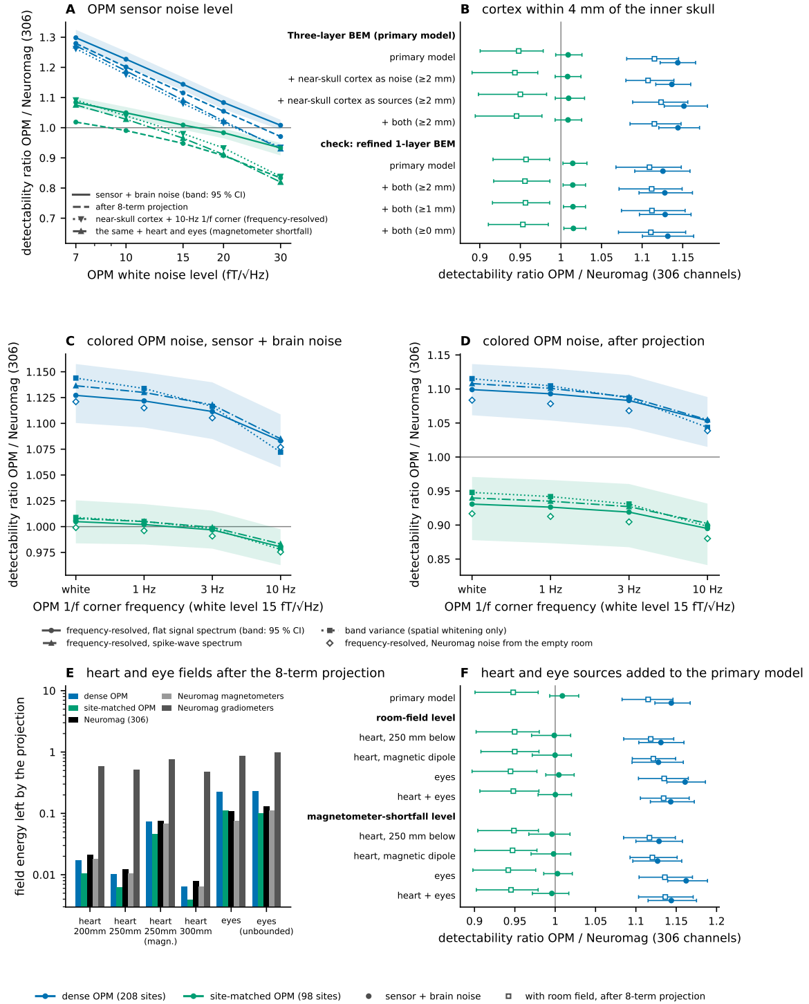
Fig. S5. Sensitivity of the adult comparison to the noise model. Median ratio OPM/Neuromag (306 channels) over the 7,661 targets for the dense (208 sites, blue) and site-matched (98 sites, green) OPM arrays, with 95 % parcel-bootstrap bands or bars. In B and F, filled circles, sensor plus brain noise; open squares, room field projected out. (A) Ratio against OPM white noise (7, 10, 15, 20 and 30 fT/√Hz): primary model (solid, band); projected (dashed); near-skull cortex with a 10-Hz 1/f corner, frequency-resolved detector (dotted, inverted triangles); the same with heart and eyes at the magnetometer-shortfall level (dash-dotted, triangles). (B) Near-skull cortex as noise, sources or both (three-layer BEM), and down to the inner skull (refined single-compartment BEM). (C, D) Ratio at 15 fT/√Hz against the 1/f corner, unprojected (C) and projected (D): frequency-resolved detector with flat (circles, band) or spike-wave (triangles) signal spectrum, band-variance detector (squares, dotted), and frequency-resolved detector with Neuromag's empty-room noise (open diamonds). (E) Share of cardiac and ocular field energy left after the projection, per array and for Neuromag's magnetometers and gradiometers (logarithmic axis). (F) Ratio with these sources added at the room field's level and at the shortfall level.
