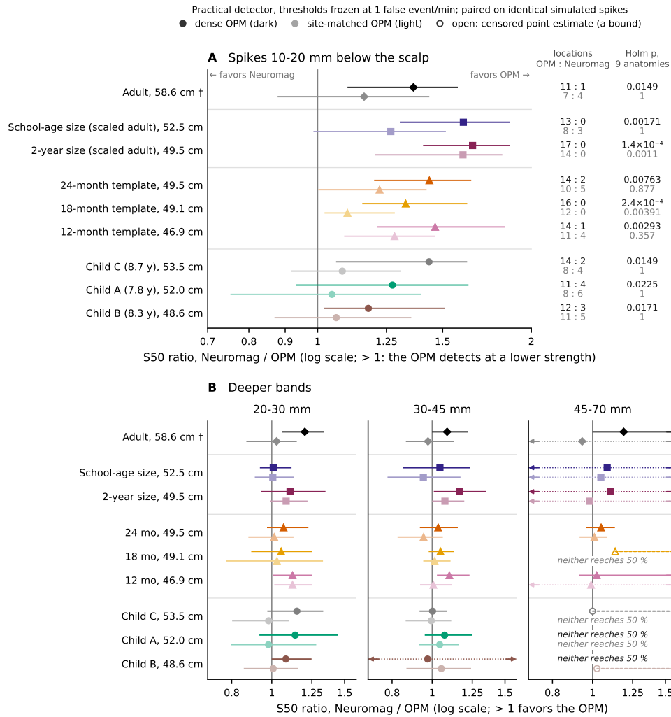
Fig. S12. Simulated interictal spikes, exploratory run. Paired S50 ratio Neuromag (306 channels) / OPM, practical detector; logarithmic axis with a line at 1 (above 1: the OPM detects at a lower strength). (A) Spikes 10–20 mm below the scalp, with the locations favoring each system and the sign-flip p Holm-adjusted over the 9 anatomies for each array separately; this endpoint was chosen after the analyses. (B) The deeper bands. Dark markers: dense OPM array; light markers: site-matched OPM array. Lines: 95 % bootstrap intervals over the 18 locations per band and anatomy (324 focal events). Arrows: open interval ends (resamples outside the tested 10–320 nAm); dotted lines: intervals open at both ends; open markers: censored point estimates (with a dashed arrow: Neuromag does not reach half detection, so the ratio lies above the bound); “neither reaches 50 %”: no estimate. Dagger: the adult at its measured head position; other heads at top contact. OPM, optically pumped magnetometer.
