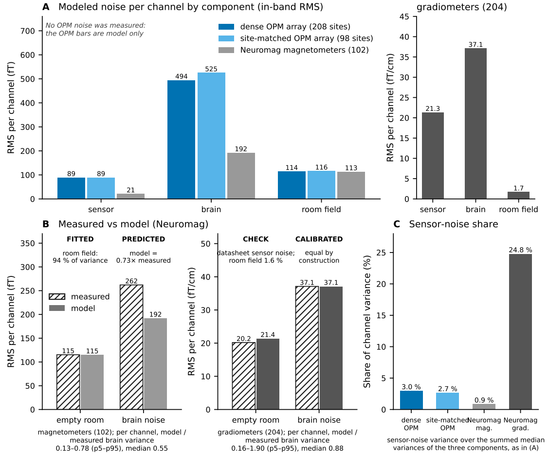
Fig. S2. The noise budget and what is fitted, checked, calibrated and predicted. (A) Modeled in-band RMS noise per channel by component (sensor noise, cortical background, room field), the square root of each component's median channel variance (RMS values do not add), for the dense OPM array (208 sites), the site-matched OPM array (98 sites) and Neuromag's 102 magnetometers; the 204 gradiometers on their own fT/cm axis. The OPM bars are model only. (B) Measured Neuromag quantities against the model: the empty-room level (magnetometers, a fit; gradiometers, a check) and the brain noise (magnetometers, a prediction; gradiometers, calibrated). Labels under the panels give the median and the 5th to 95th percentiles over channels of the modeled-to-measured brain-noise variance; the covariance check of Section S3.4 excludes the bad channel, so its gradiometer range differs slightly. (C) The sensor-noise share of the in-band variance with brain noise and room field. RMS, root-mean-square.
