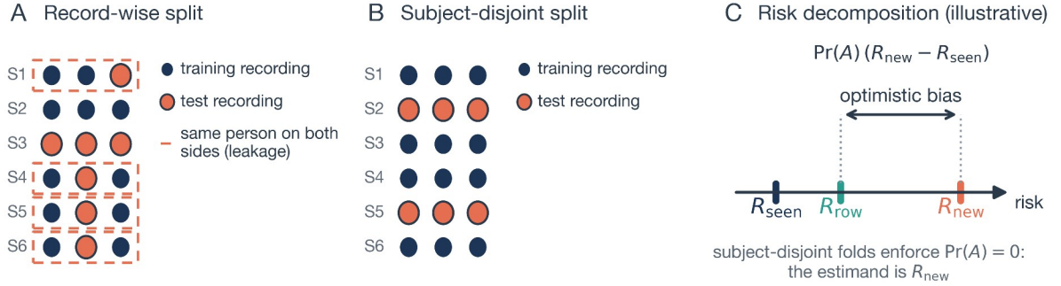
150 Figure 2. Schematic illustration of evaluation leakage with repeated recordings. (A) A record-wise split assigns 151 individual recordings to training or test sets, so several subjects (dashed outlines) appear on both sides and the test 152 set is not independent of training identities. (B) A subject-disjoint split assigns all recordings of a subject jointly. (C) 153 Consequence of Equation (20): the record-wise estimate R_{row} interpolates between the easier seen-person risk 154 R_{seen} and the deployment-relevant unseen-person risk R_{new} , drawn for an illustrative Pr(A)=0.65 ; the arrow 155 marks the optimistic bias of magnitude Pr(A)(R_{new} - R_{seen}) .
