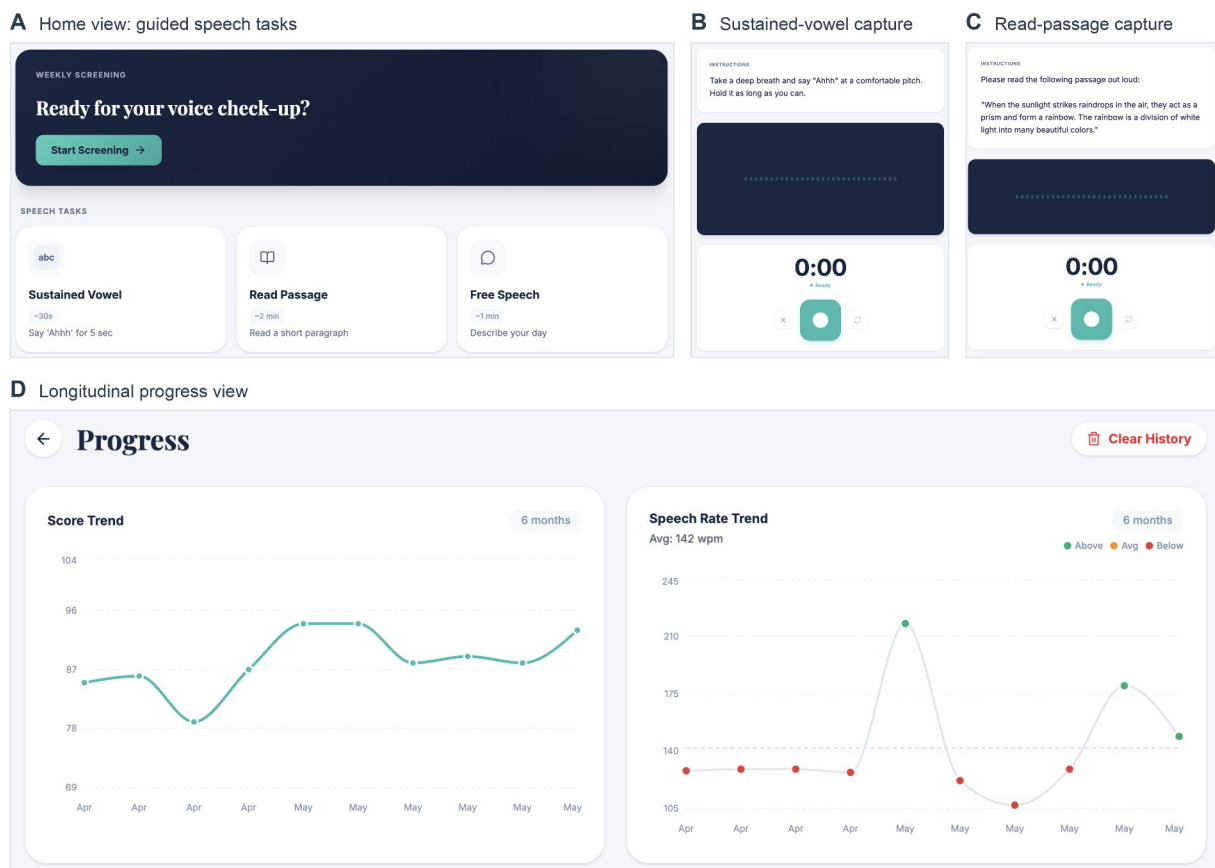
Figure 9. VoxNeuro web application (publicly accessible research-stage prototype). (A) Home view listing the three guided speech tasks. (B) Sustained-vowel capture screen. (C) Read-passage capture screen showing an excerpt from the Rainbow Passage. (D) Longitudinal progress view with illustrative entries. The application requires only a commodity microphone and a web browser; no application-collected data were used in the analyses reported here.
