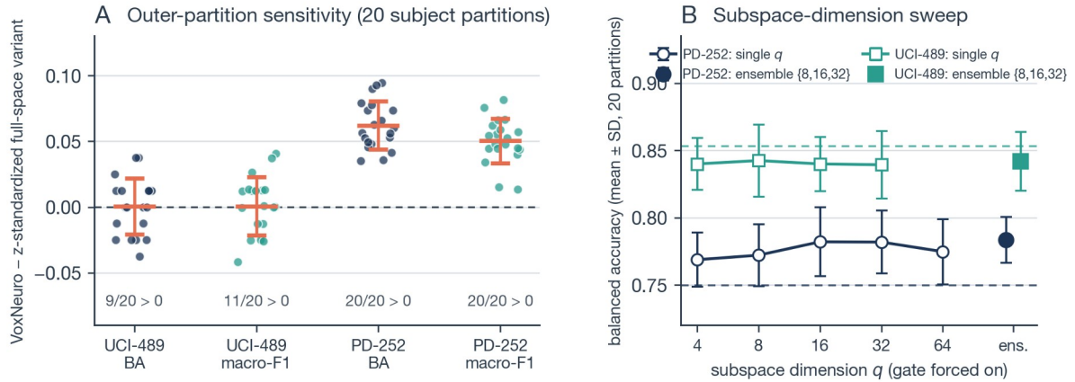
Figure 8. Sensitivity of VoxNeuro to the outer subject partition and to the subspace dimension. (A) Paired differences between VoxNeuro and its z-standardized full-space ablation across 20 alternative outer subject
