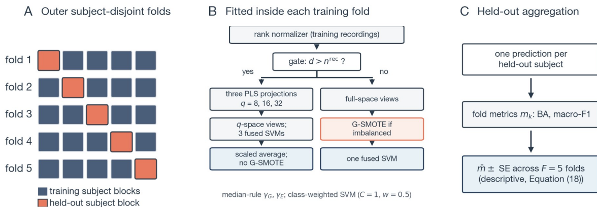
380 Figure 5. Evaluation protocol. (A) Five-fold subject-disjoint partition; in each outer fold one subject block (orange) 381 is held out and never influences any fitted component. (B) Everything that learns from data is fitted inside the 382 training fold only: the rank normalizer, then either the supervised-subspace branch (dimensionality gate active: 383 PLS projections, q -space views, three SVMs averaged after scaling; no synthetic subjects) or the full-space branch 384 (gate inactive: full-space views, conditional G-SMOTE in imbalanced folds, one SVM), with median-rule kernel 385 coefficients in both branches. (C) Exactly one prediction is issued per held-out subject, fold metrics are computed 386 at the subject level, and Equation (18) aggregates them descriptively.
