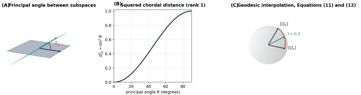
Figure 4. The geometry behind Equations (5), (6), (11), and (12), drawn for illustrative toy subspaces. (A) The first principal angle \theta_{ij,1} between two subspaces of \mathbb{R}^3 . (B) Exact rank-one relation between a principal angle and the squared chordal distance, d_{\text{ch}}^2 = \sin^2 \theta . (C) A geodesic path computed with Equations (11) and (12) between two one-dimensional subspaces [Q_a] and [Q_b] ; every interpolated frame in the drawn path satisfies Q_{\text{syn}}(t)^T Q_{\text{syn}}(t) = I_r to machine precision, consistent with Proposition 2.
