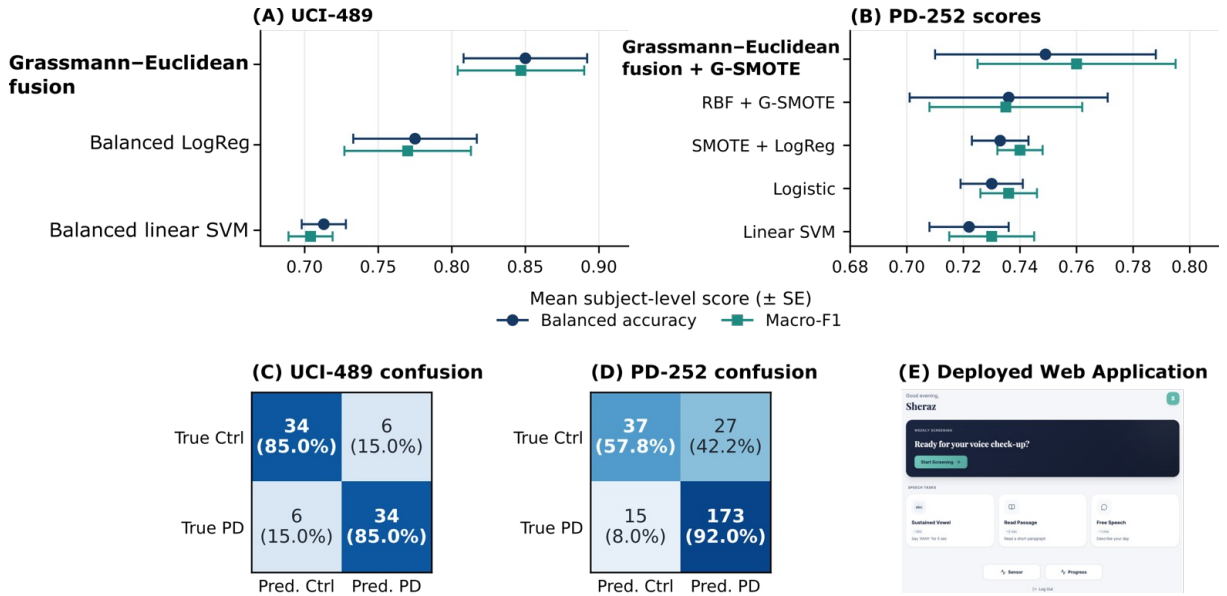
Figure 6. Subject-level speech results. Whiskers denote standard error across five outer folds. (A) On balanced UCI-489, the Grassmann–Euclidean fusion model attained the highest mean balanced accuracy and macro-F1 among the audited comparators. (B) On high-dimensional, imbalanced PD-252, fusion with G-SMOTE attained the highest mean balanced accuracy and macro-F1; RBF + G-SMOTE is the matched nonlinear Euclidean ablation and SMOTE + LogReg is SMOTE with logistic regression. Balanced LogReg and Logistic denote class-weighted logistic regression; Balanced linear SVM and Linear SVM denote class-weighted linear SVM. (C,D) Pooled out-of-fold
