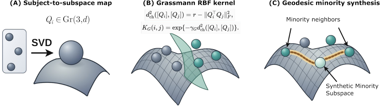
Figure 3. Geometric interpretation of the VoxNeuro representation, adapted from the project poster. (A) Three repeated recordings are mapped by a thin SVD to a fixed-rank representation on \text{Gr}(3, d) . (B) Squared chordal distance and the associated Gaussian Grassmann radial-basis-function kernel compare subjects independently of the arbitrary orthonormal basis selected for each subspace. (C) Minority subjects are synthesized along a Grassmann geodesic rather than by row-wise Euclidean interpolation.
