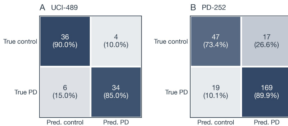
Figure 7. Pooled out-of-fold confusion matrices of VoxNeuro for (A) UCI-489 and (B) PD-252 at the reference partition, containing one prediction per subject; percentages are normalized within the true class. The model generated no synthetic subjects on either evaluated cohort, so the counts do not depend on an augmentation seed; they are reference-partition estimates and not externally validated operating characteristics.
