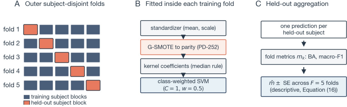
Figure 5. Evaluation protocol. (A) Five-fold subject-disjoint partition; in each outer fold one subject block (orange) is held out and never influences any fitted component. (B) Everything that learns from data—the standardizer, G-SMOTE, the kernel coefficients, and the SVM—is fitted inside the training fold only. (C) Exactly one prediction is issued per held-out subject, fold metrics are computed at the subject level, and Equation (16) aggregates them descriptively.
