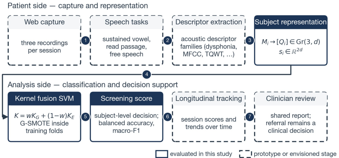
Figure 10. Envisioned deployment workflow of the VoxNeuro prototype. Solid boxes mark the components evaluated in this study on the two public cohorts (subject representation, kernel fusion with G-SMOTE, and subject-level scoring); dashed boxes mark capture and decision-support stages of the research-stage prototype that were not evaluated here. Descriptor extraction in this study used the dataset-provided engineered features, and any referral decision remains a clinical judgement.
