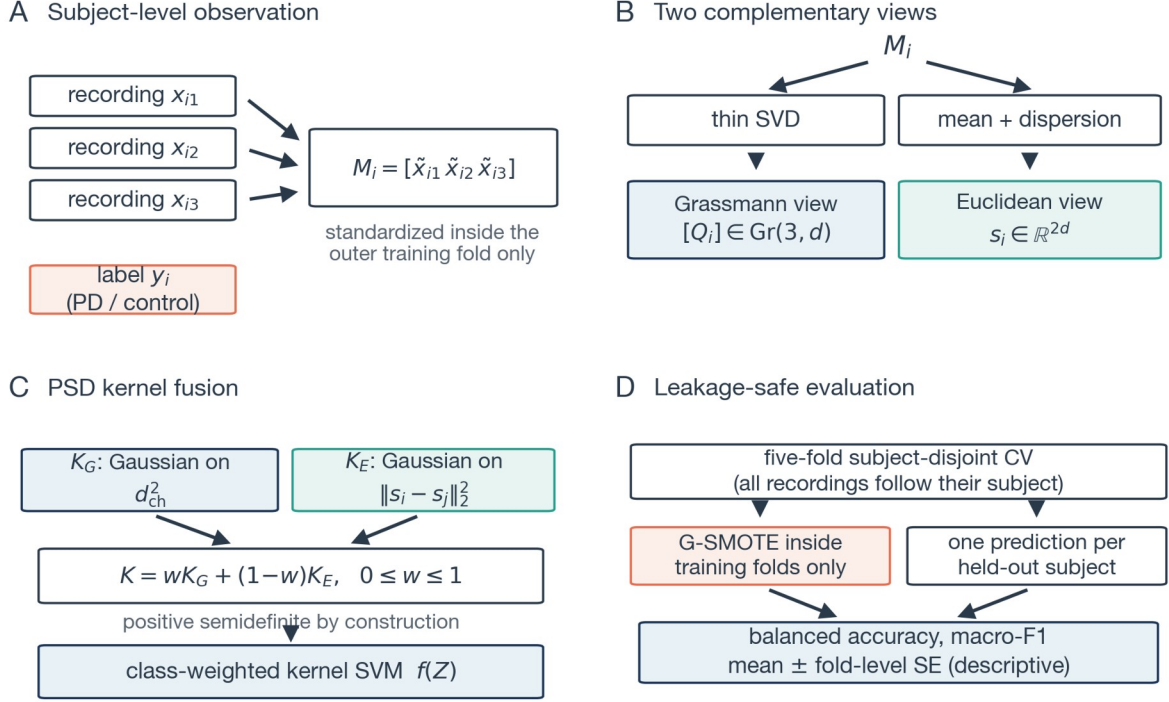
Figure 1. Schematic overview of the VoxNeuro framework. (A) Each subject contributes three repeated recordings and one diagnostic label; the recordings are standardized with statistics estimated inside the outer training fold only and stacked into a matrix M_i . (B) A thin singular value decomposition (SVD) yields the Grassmann view [Q_i] , while coordinate-wise mean and dispersion yield the Euclidean view s_i . (C) Gaussian kernels on the two views are combined into a positive-semidefinite (PSD) fused kernel feeding a class-weighted support vector machine (SVM). (D) Evaluation is five-fold subject-disjoint cross-validation (CV); Grassmann-geodesic synthetic minority oversampling (G-SMOTE) operates inside training folds only, and fold scores are summarized as mean \pm standard error (SE). PD, Parkinson’s disease.
