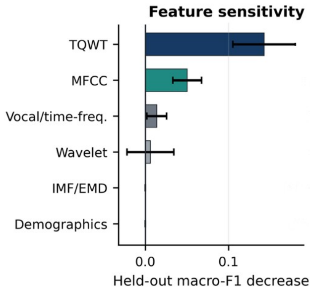
Figure 8. PD-252 feature-family permutation sensitivity on the Euclidean summary view. Positive values denote a decrease in held-out macro-F1 after permutation, and whiskers denote fold-level standard error. TQWT denotes tunable Q-factor wavelet transform; MFCC denotes Mel-frequency cepstral coefficients; IMF/EMD denotes intrinsic mode function/empirical mode decomposition; Demographics denotes the dataset-provided sex/gender covariate.
