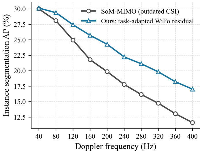
(a) AP
