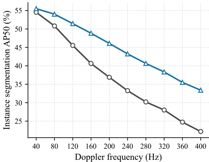
(b) AP50
