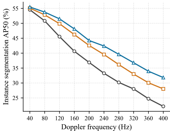
(b) AP50
