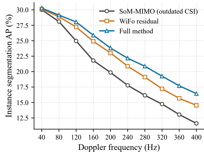
(a) AP
