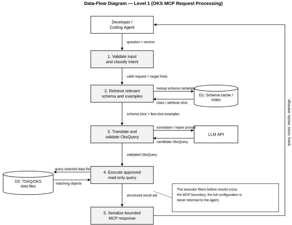
Figure 3.5: Level-1 data-flow diagram for OKS MCP request processing.
