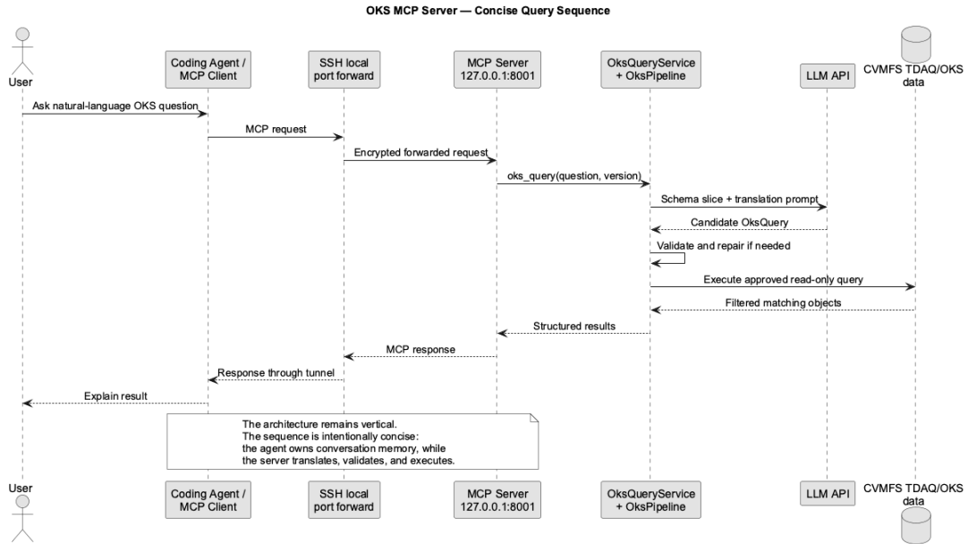
Figure 3.4: Concise sequence of operations for an MCP query request.
