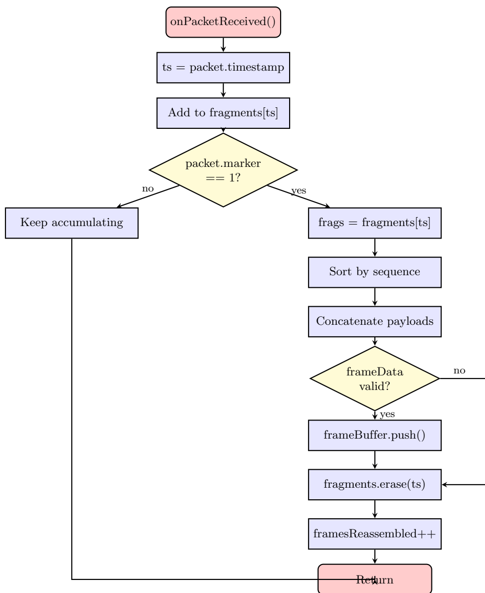
Figure 11: Flowchart of Frame Reassembly algorithm
