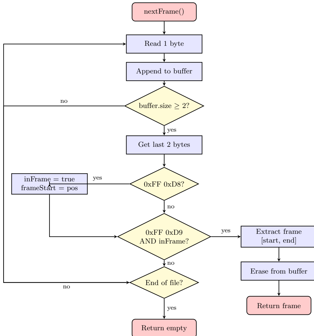
Figure 9: Flowchart of MJPEG frame extraction algorithm
