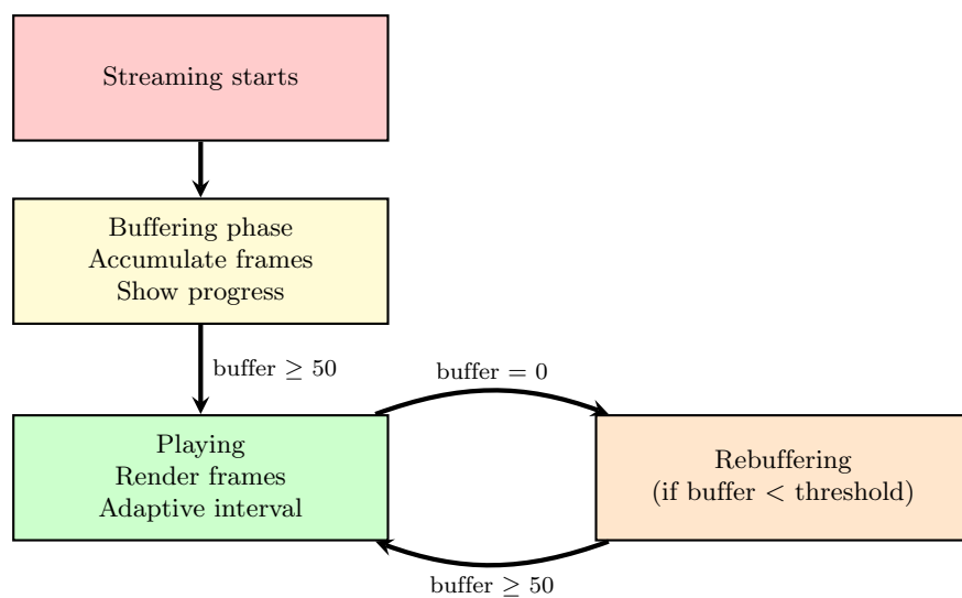
Figure 13: State flow of prebuffering mechanism
