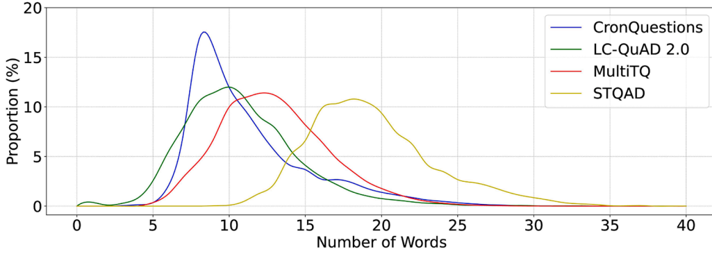
Fig. 3. Length distribution of datasets.
