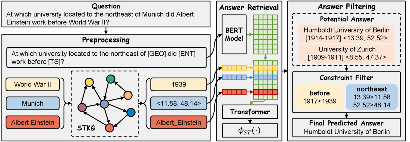
Fig. 4. Model architecture of STCQA.
