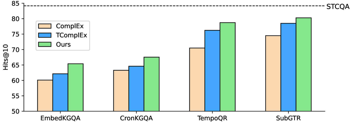
Fig. 5. Performance (Hits@10) of embedding-based KGQA baselines on STQAD using different embedding models.
