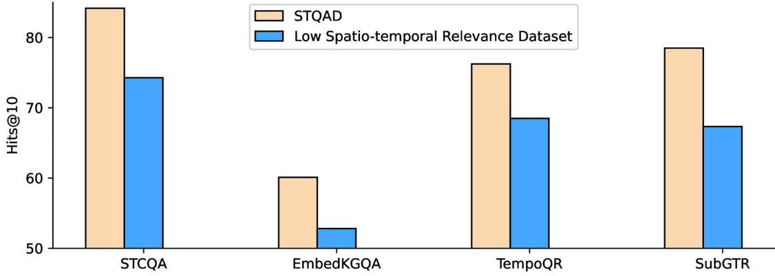
Fig. 6. Model performance (Hits@10) on different spatio-temporal constraint relevance dataset.
