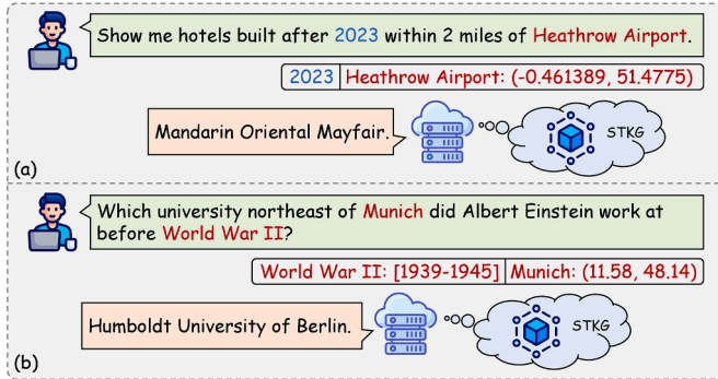
Fig. 1. The user request in Fig. 1(a) involves the calculation of distance, while Fig. 1(b) addresses the comparison of orientation. In the question presented in Fig. 1(a), temporal information 2023 is explicitly provided (in blue). The question in Fig. 1(b) is more challenging, as neither the timestamp nor the geographic coordinates are explicitly provided (in red).
