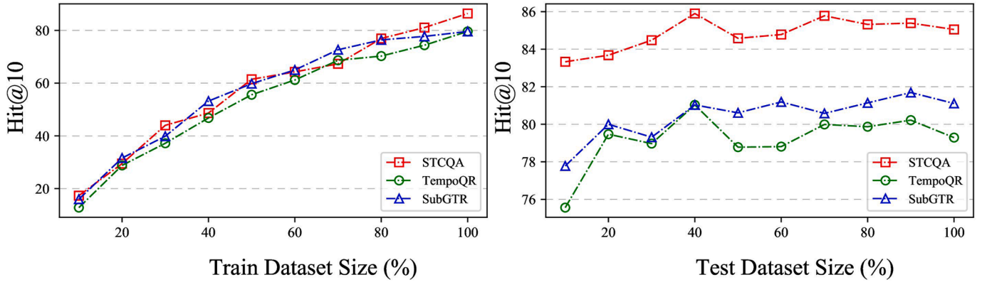
Fig. 7. Model performance (Hits@10) vs. dataset size for STCQA, TempoQR and SubGTR.
