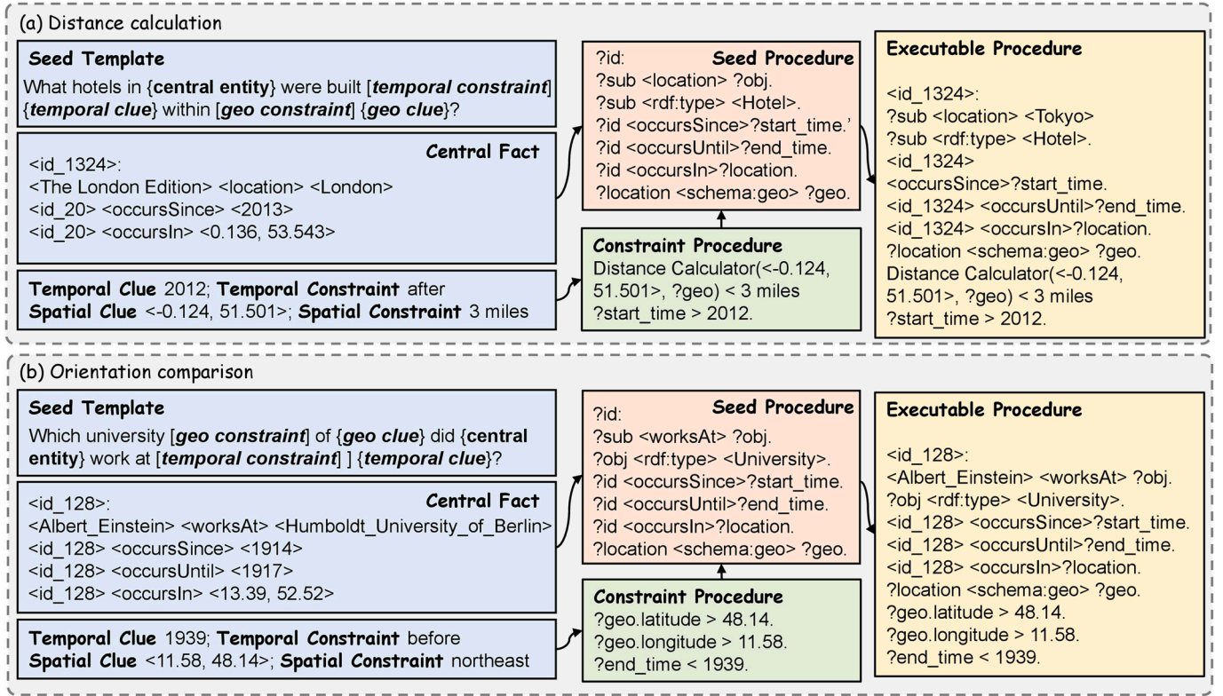
Fig. A.8. Examples of our seed procedures. Example (a) illustrates distance calculation. We use the Distance Calculator based on the Haversine formula to verify geographical constraints. Example (b) demonstrates orientation comparison, where our program can compare all constraints.
