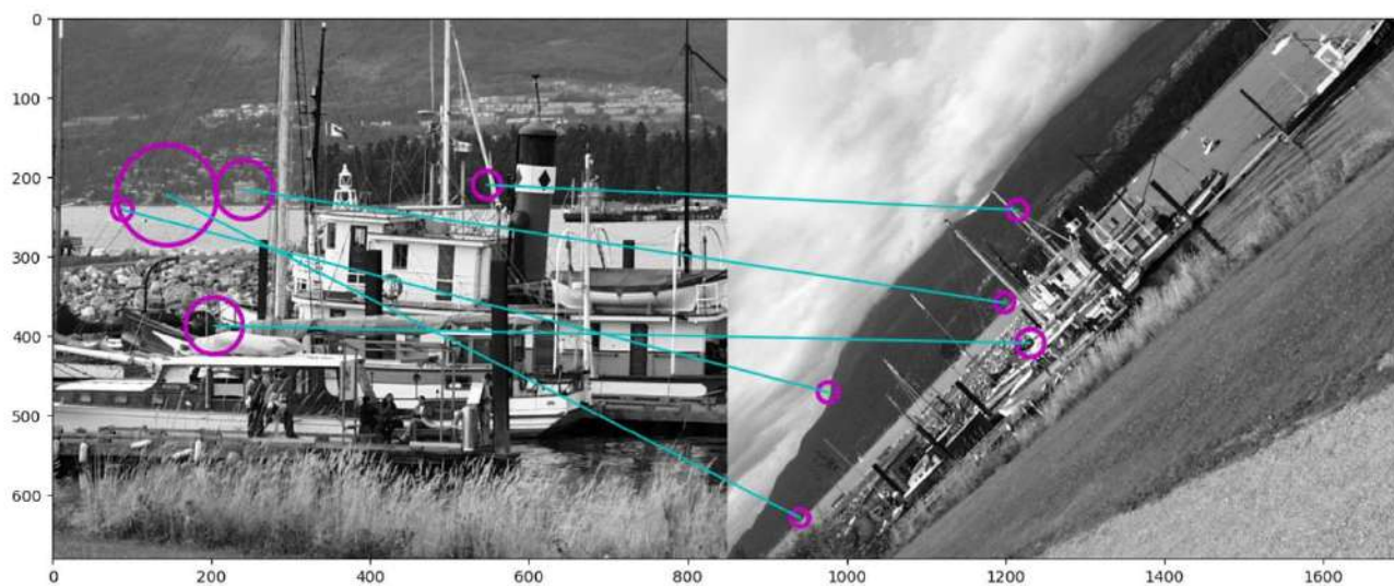
Top 5 mutual nearest neighbors of SURF features
