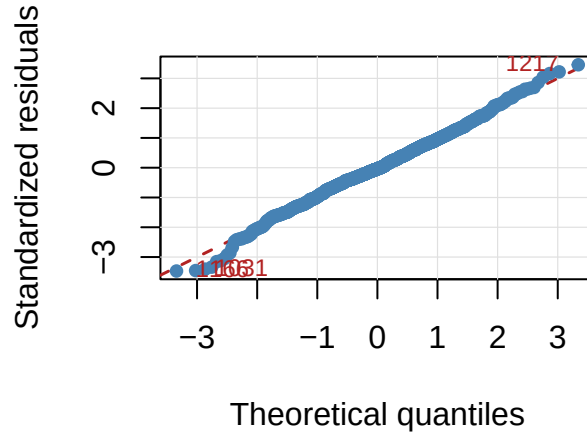
Normal Q-Q – OLS standardized resid
