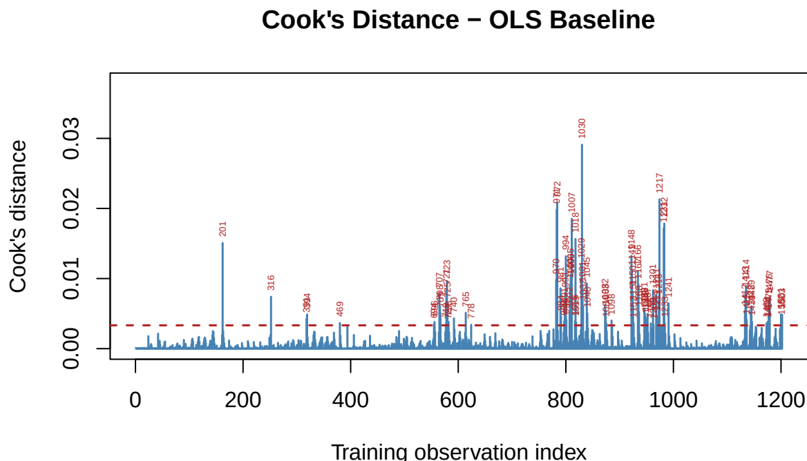
Figure 2: Cook’s distance for the OLS fit. Bars above the dashed 4/n threshold are flagged as influential; each flagged bar is labelled with its row number in the original airfoil_self_noise data, not its training position.
