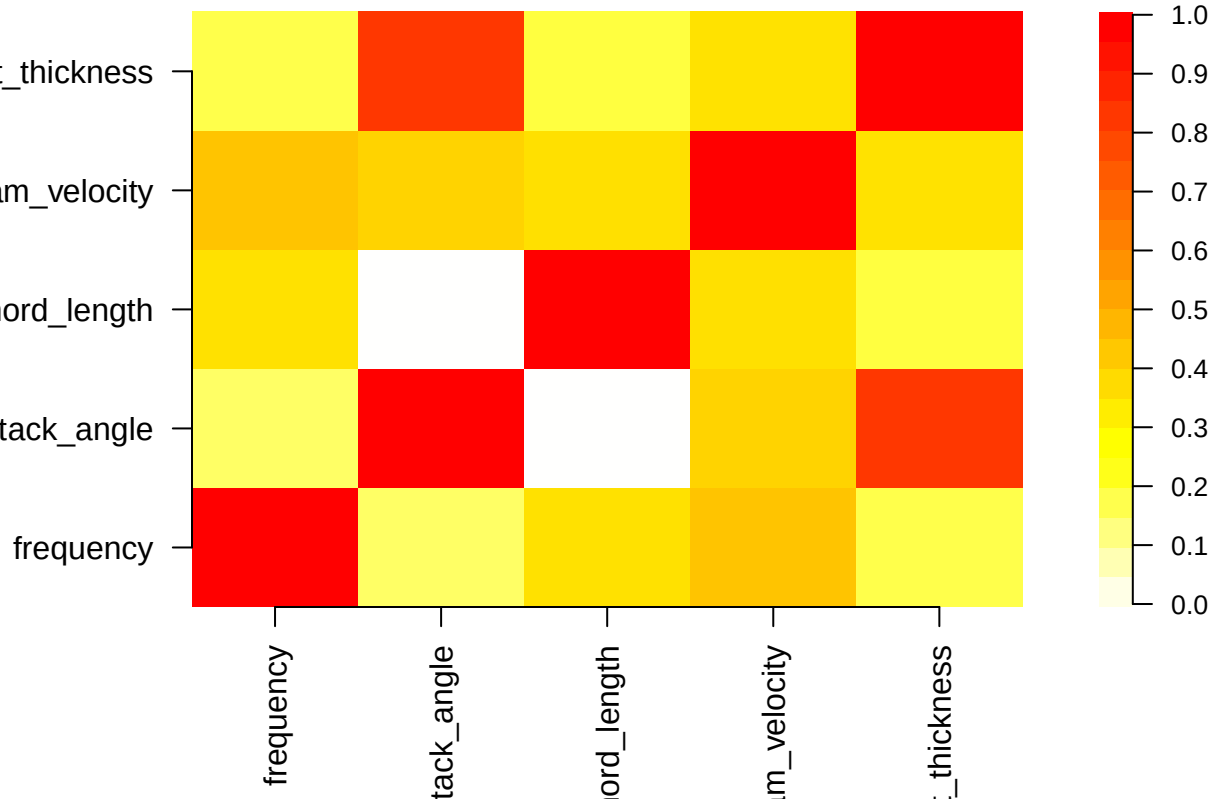
Correlation Heatmap of Predictors
