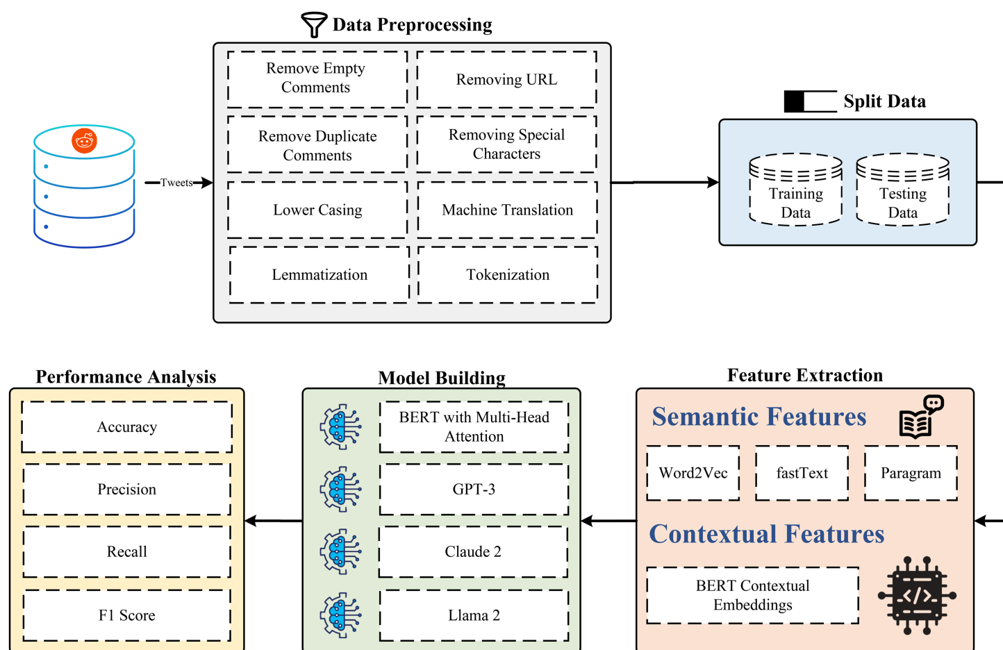
Fig 4. Architecture of the proposed sarcasm detection framework. The pipeline integrates preprocessing (translation, normalization, cleaning), feature extraction (Word2Vec, fastText, Paragram, BERT), and model building (BERT with multi-head attention, GPT-3, Claude-2, Llama-2), followed by evaluation.
