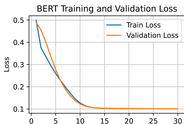
Fig 6. Training and validation loss curves of BERT showing stable convergence during sarcasm detection.
