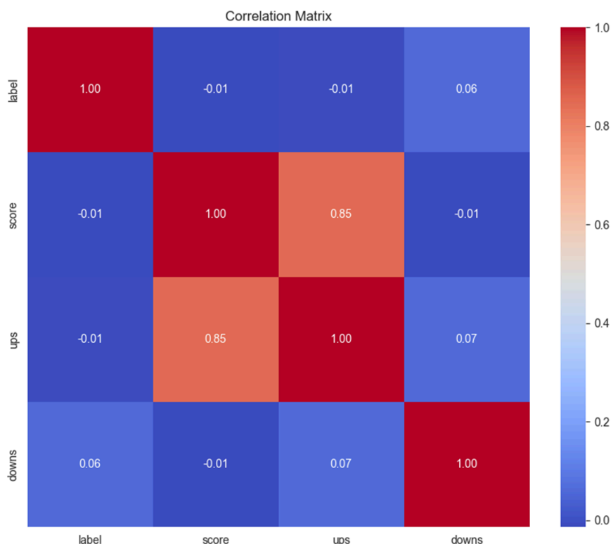
Fig 1. Correlation heatmap showing relationships among SARC metadata features. Upvotes ('ups') strongly correlate with the overall score, while downvotes ('downs') exhibit a weaker or negative association, illustrating how community reactions shape the visibility of sarcastic content.
