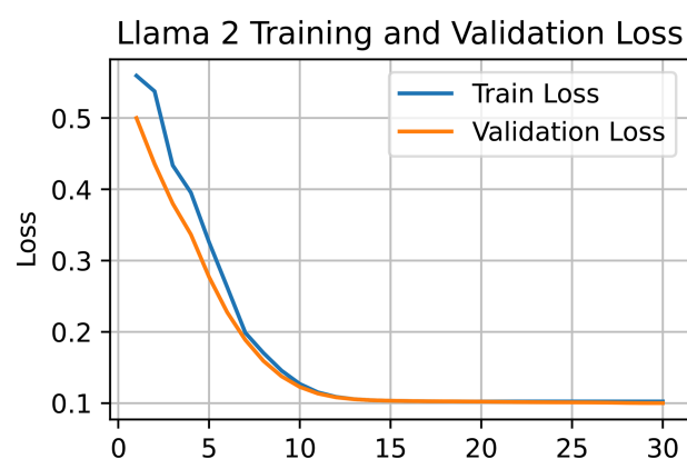
Fig 8. Training and validation loss curves of Llama-2 demonstrating consistent and balanced convergence behavior.
