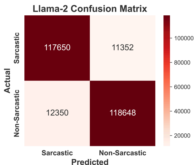
Fig 12. Confusion matrix of Llama-2 model reflecting competitive performance with moderate misclassification rates.
