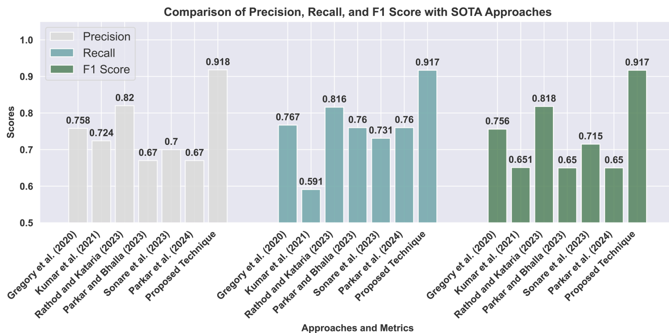
Fig 13. Precision, recall, and F1 score comparison between the proposed method and prior approaches. The fine-tuned BERT with multi-head attention significantly outperforms state-of-the-art baselines.
