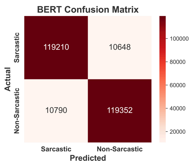
Fig 9. Confusion matrix of BERT model showing high accuracy with minimal false positives and false negatives.
