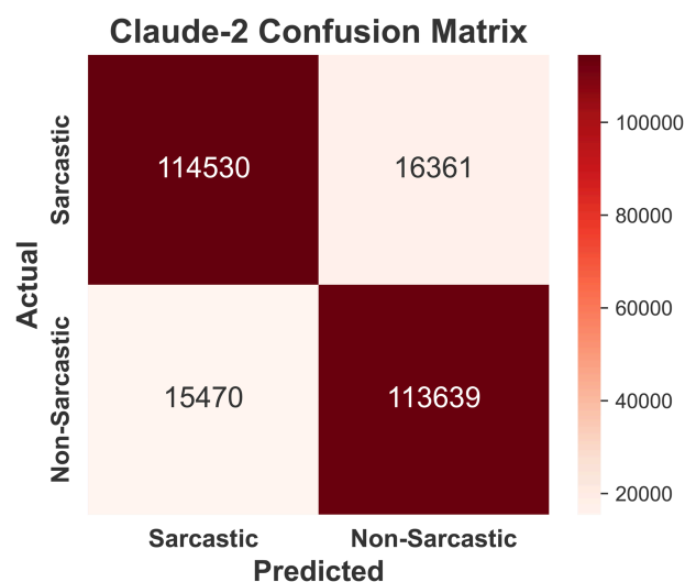
Fig 11. Confusion matrix of Claude-2 model illustrating greater false positives and false negatives, reducing detection reliability.
