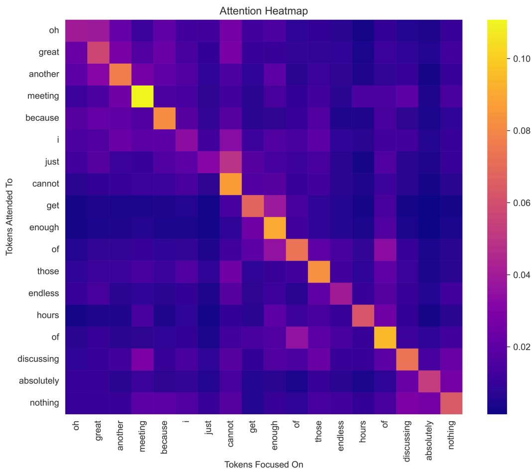
Fig 14. Attention heatmap from the fine-tuned BERT model, showing how multi-head attention highlights key tokens in a sarcastic sentence (e.g., ‘oh great,’ ‘another meeting,’ ‘endless hours’). The visualization demonstrates the model’s ability to focus on lexical cues and contextual dependencies that signal sarcasm, providing interpretability into how the model distinguishes sarcastic from non-sarcastic text.
