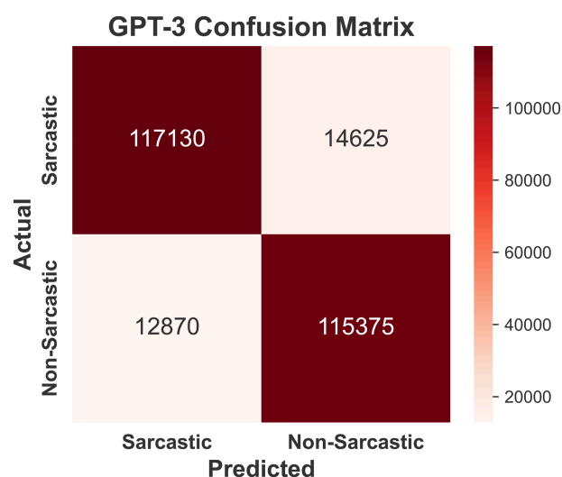
Fig 10. Confusion matrix of GPT-3 model indicating balanced performance but with higher misclassifications than BERT.
