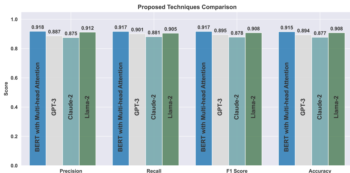
Fig 5. Comparison of sarcasm detection performance across BERT, GPT-3, Claude-2, and Llama-2 on the SARC dataset. BERT with multi-head attention achieves state-of-the-art accuracy and F1 scores.
