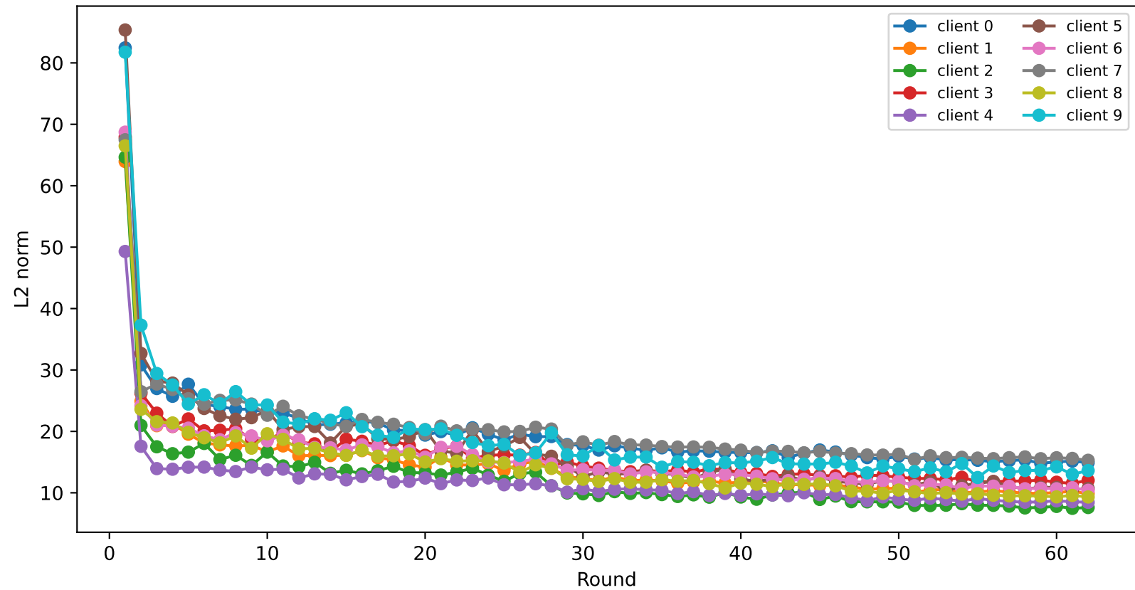
Client update L2 norms
