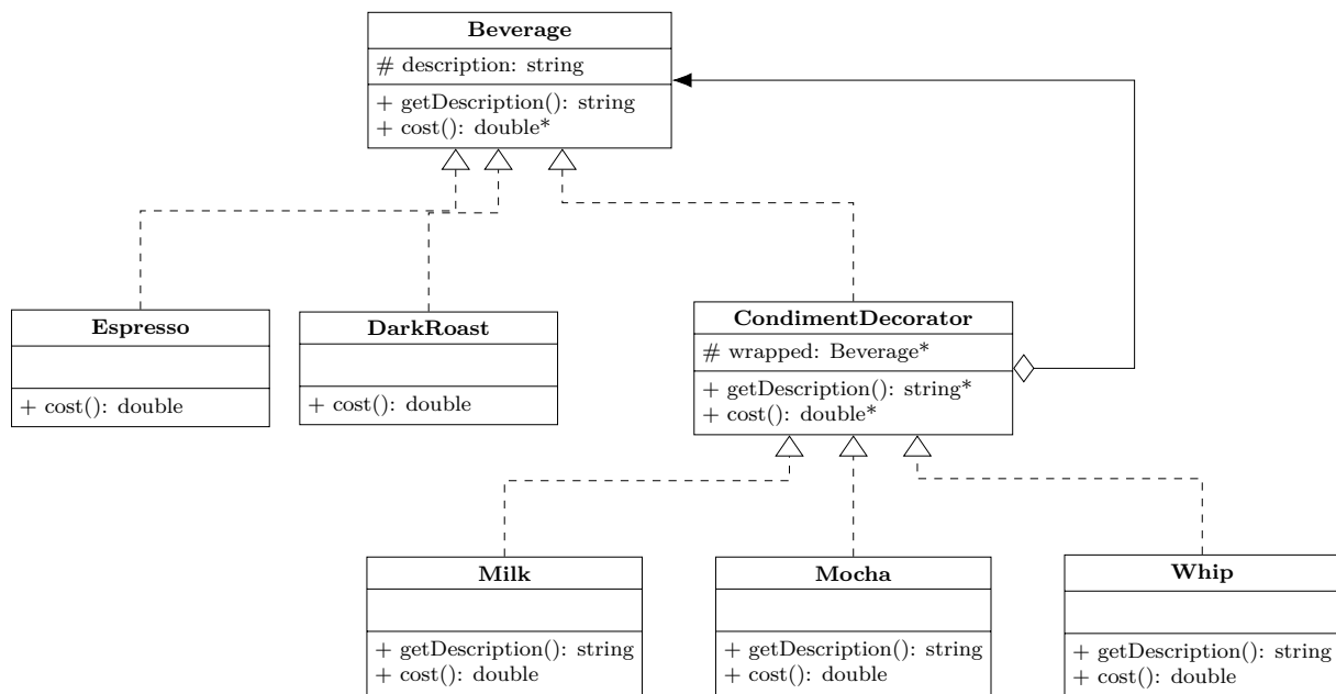
Figure 2.2: Decorator pattern applied to the coffee beverage customization system.
