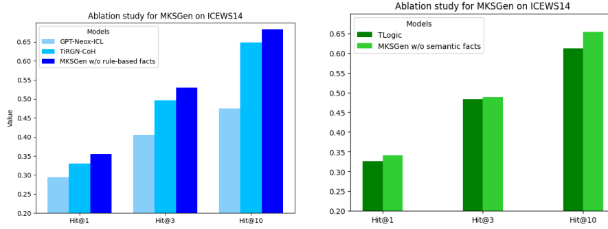
Fig. 2: Ablation studies.
