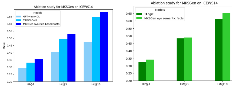
Fig. 2: Ablation studies.
