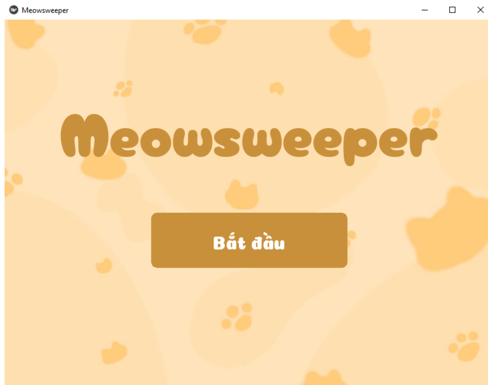
Title Screen
