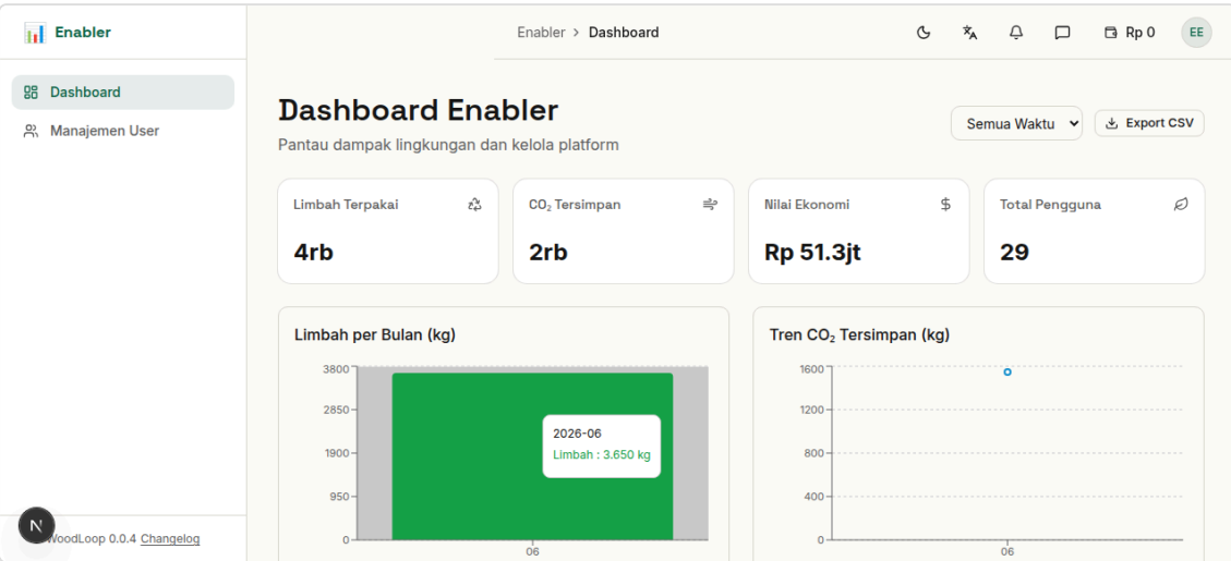
Gambar 3.1 — Dashboard Enabler
