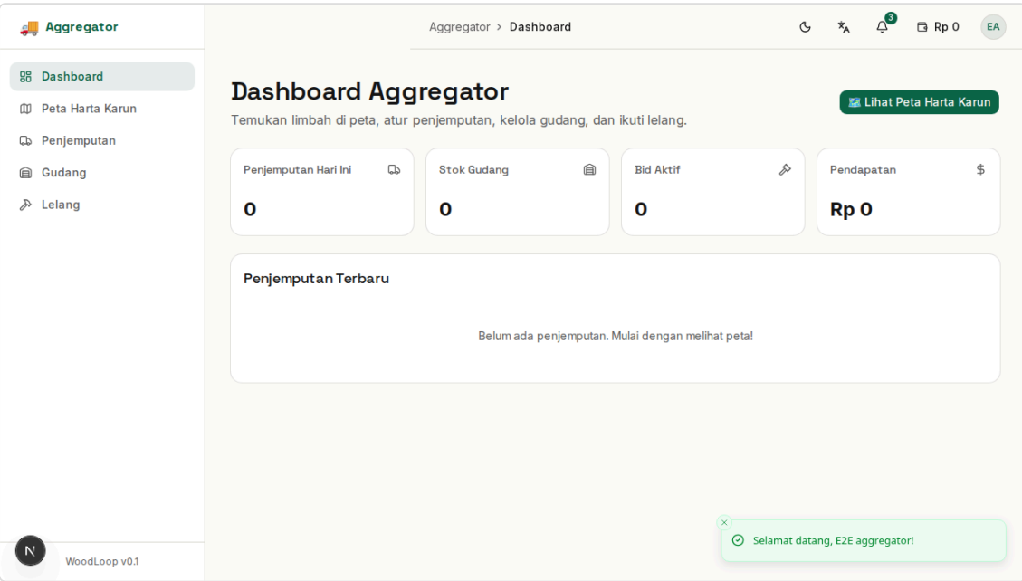
Gambar 3.1 — Dashboard Aggregator
