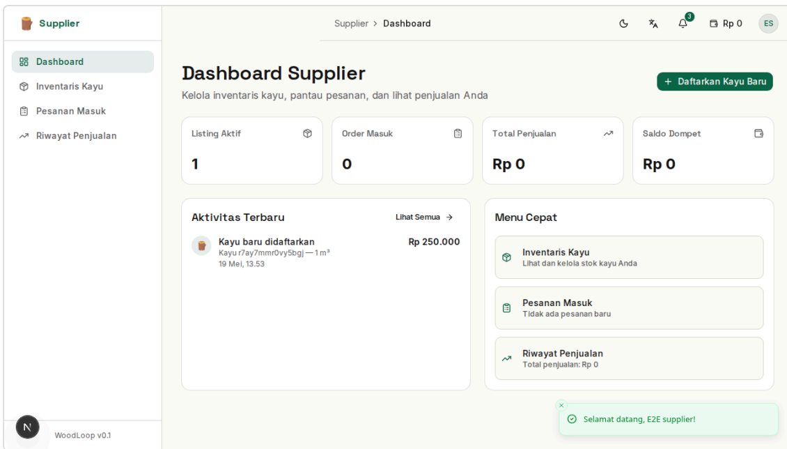
Gambar 2.1 — Dashboard Supplier
