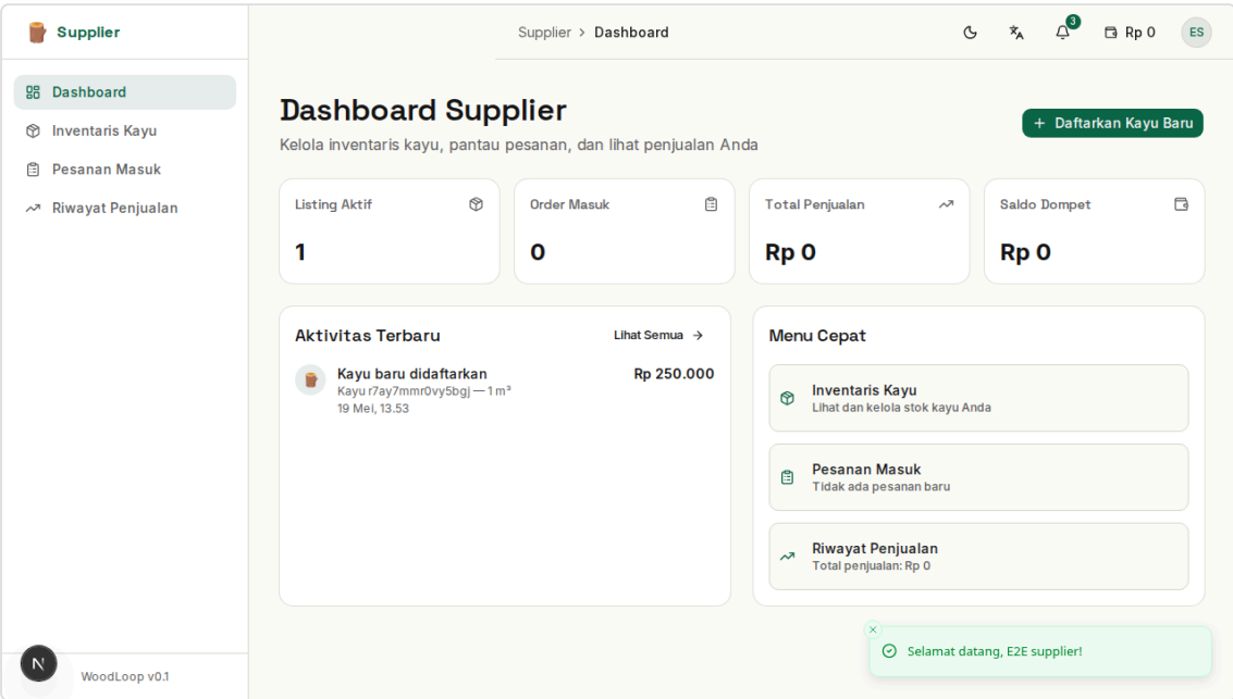
Gambar 3.1 — Dashboard Supplier
