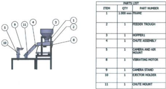
Figure 2.5: Fully fabricated mechanical assembly from the reference implementation [5], showing integrated hopper, vibrating feeder, chute, and frame structure. This mechanical subsystem forms the foundation upon which the improved imaging and control systems are built.
