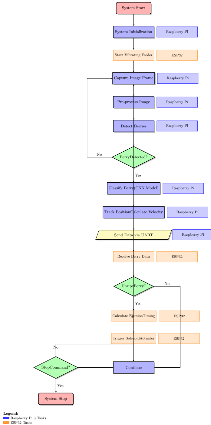
Figure 3.9: System control flow: task distribution between Raspberry Pi 4 (inference and tracking) and ESP32 (actuation, timing, and PWM control)
