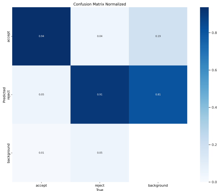
Figure 4.8: Normalised confusion matrix on the test split showing classification accuracy for accept (ripe) and reject (unripe/semi-ripe/overripe) categories
