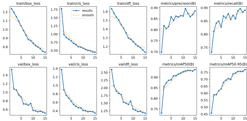
Figure 4.5: YOLOv11n training metrics over 15 epochs showing loss, precision, recall, and mAP on the binary coffee berry dataset
