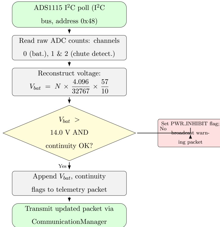
Figure 30: Power monitoring firmware flow: ADS1115 I²C readout, voltage reconstruction, arm-inhibit decision, and telemetry packet update [12, 13]. Project diagram.
