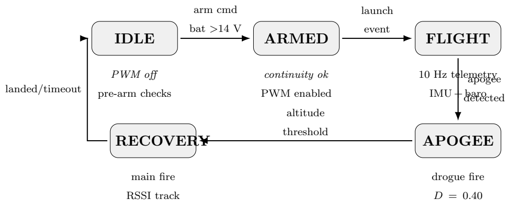
Figure 28: N4 flight firmware state machine: operational states, transitions, and per-state behaviour
