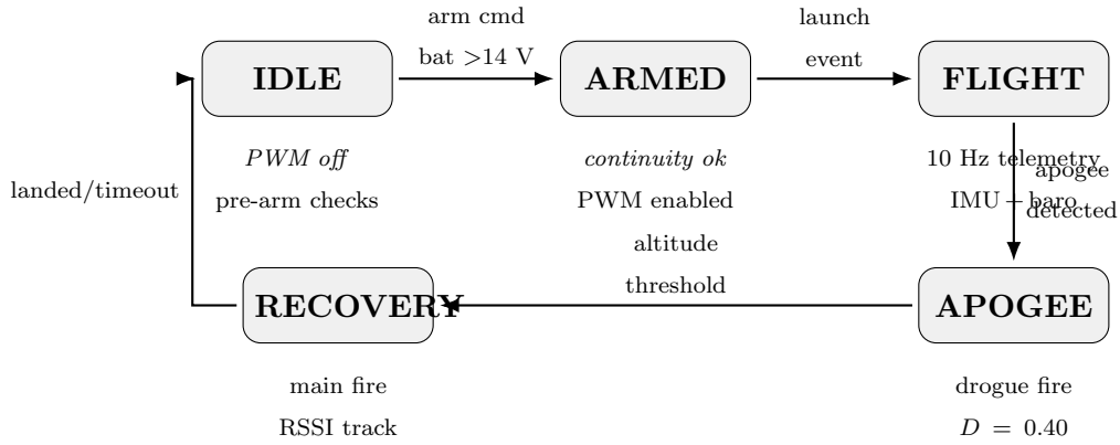
Figure 27: N4 flight firmware state machine: operational states, transitions, and per-state behaviour
