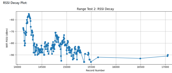
Figure 5: Beacon RSSI decay analysis showing signal degradation with distance and altitude. Project data.
