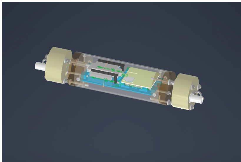
Figure 40: Full avionics bay integration showing sled mounted in cylindrical airframe section. Project fabrication.
