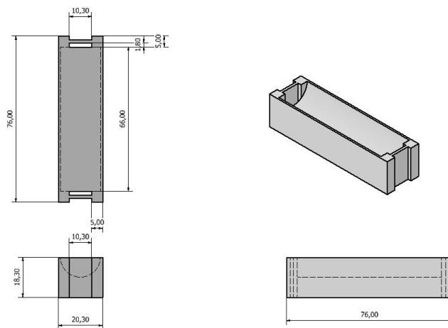
Figure 34: Raised edge battery support: orthographic views with key dimensions. Project CAD.
