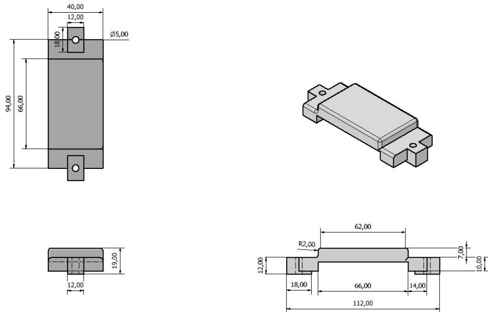
Figure 32: 18650 battery case: front, end, and top views with dimensions. Project CAD.
