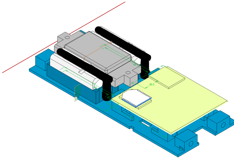
Figure 39: Avionics bay assembly: battery pack, holder, and electronics stack integrated. Project fabrication.
