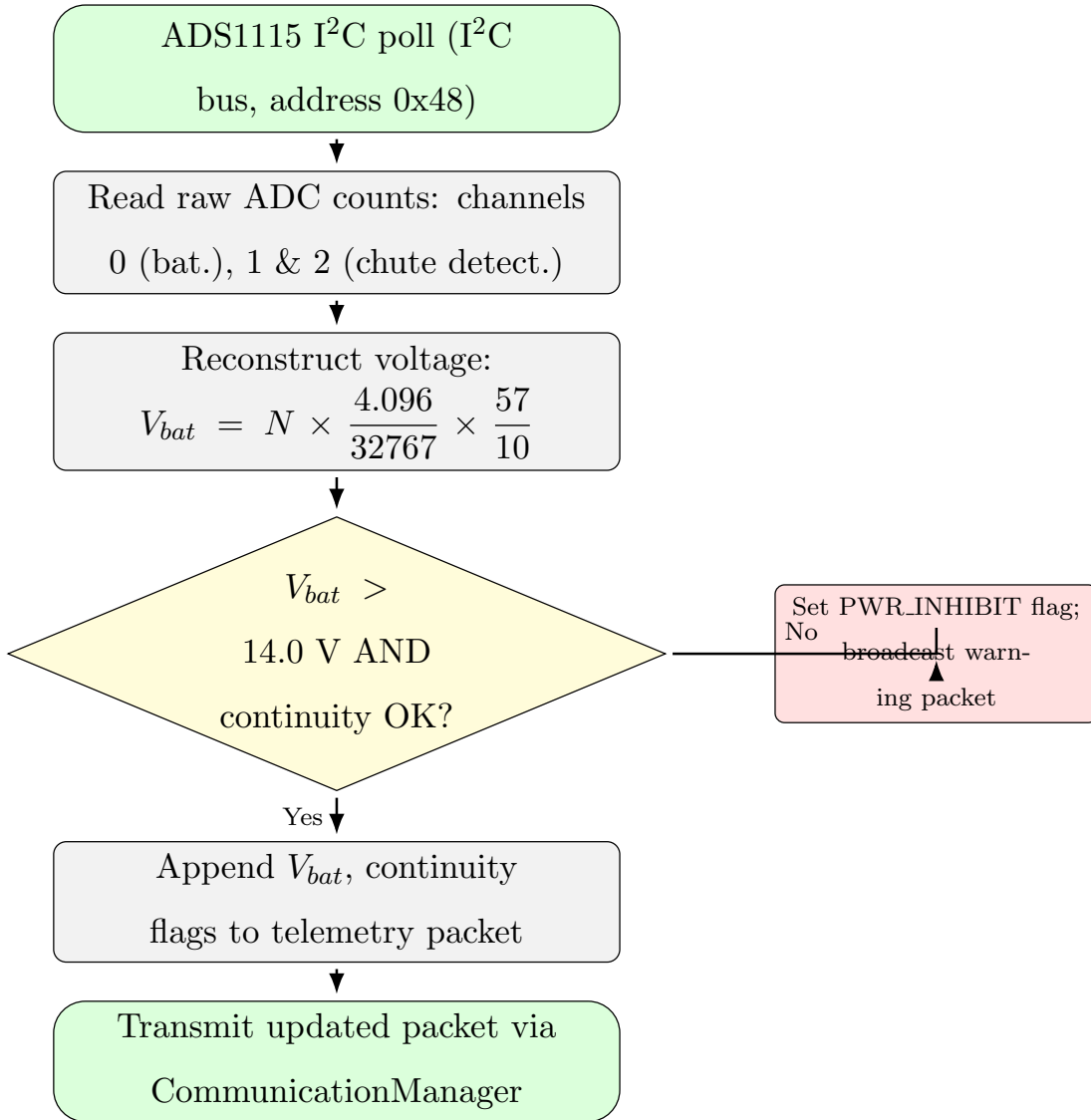
Figure 30: Power monitoring firmware flow: ADS1115 I 2 C readout, voltage reconstruction, arm-inhibit decision, and telemetry packet update [31,33]. Project diagram.
