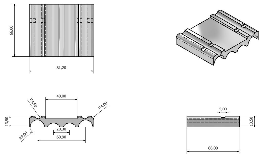
Figure 24: 18650 battery case for the stepped carrier assembly
