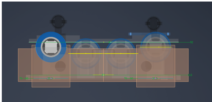
Figure 36: Threaded-rod integration: raised edge cells preserve rod clearance and structural alignment. Project CAD.
