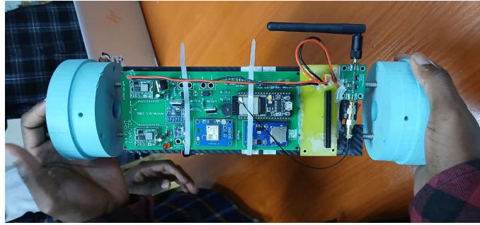
Figure 14: Assembled avionics bay with integrated battery retention and vibration isolation. Project fabrication.
