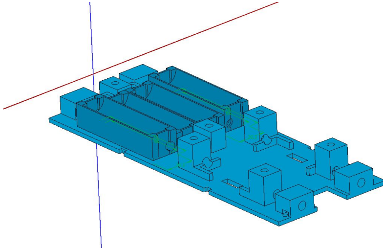
Figure 35: Flight-computer holder sled: 3D CAD model showing battery seating, rod clearances, and upper mounting platform. Project CAD.
