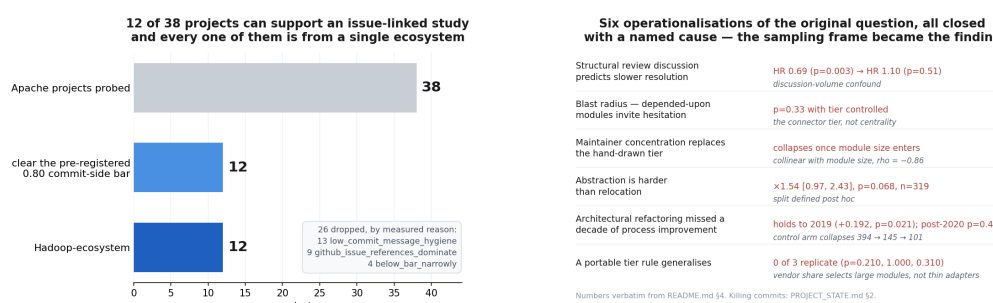
Figure 1: Corpus attrition: 38 probed projects to 12 eligible to a single ecosystem, with the six operationalisations that were tested and closed.
