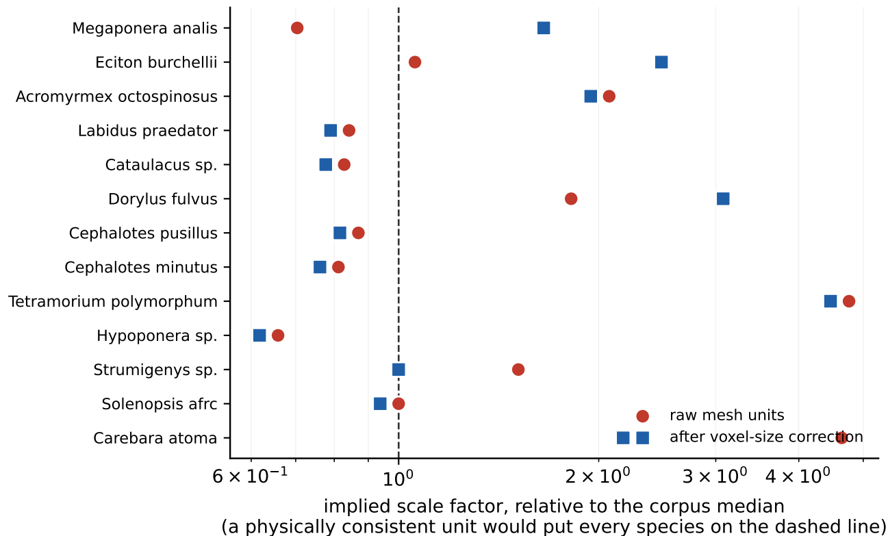
Implied physical scale disagrees by ~7× across species
