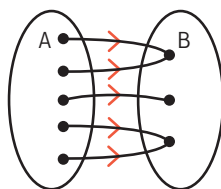
many-to-one function
