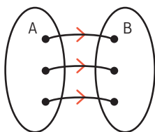
one-to-one function
