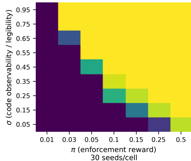
A P(active), exit OPEN ( \delta_0 = 0 )
