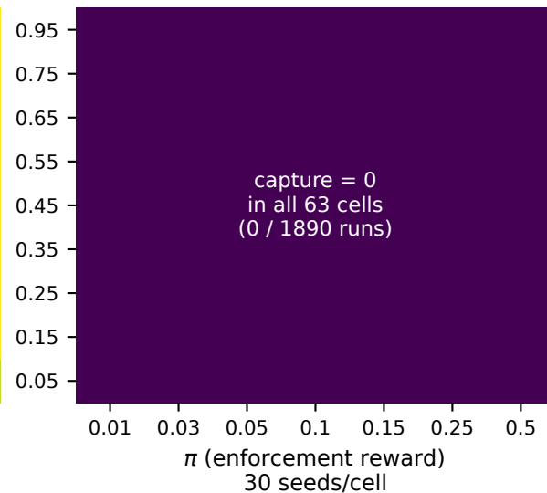
B P(capture), exit OPEN ( \delta_0 = 0 )
