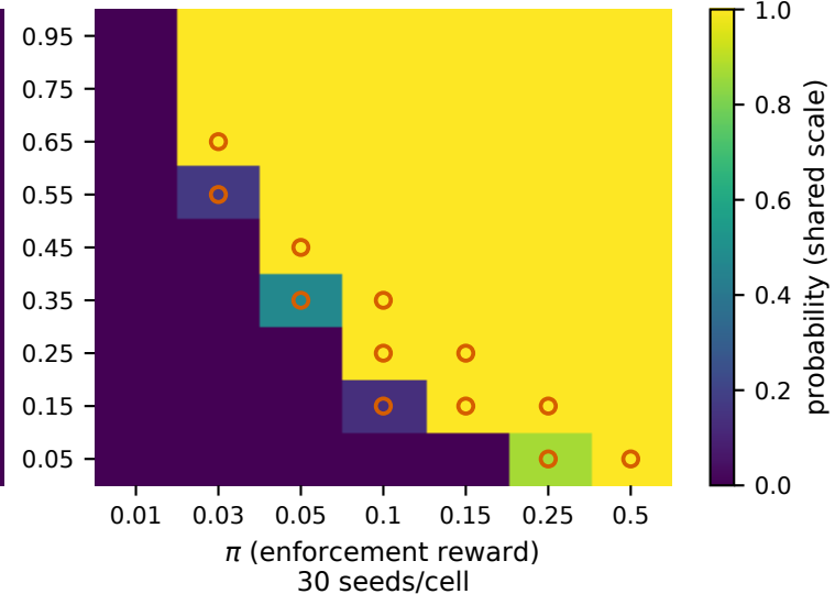
C P(capture), exit SEALED ( \delta_0 = 0.95 )
