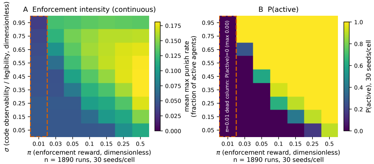
Fig 1: Activation frontier under open exit. Agent-based sweep at \delta_0 = 0 (exit open), n = 1890 runs ( 9 \sigma \times 7 \pi cells \times 30 seeds per cell). (A) Mean maximum punish rate, the continuous enforcement-intensity surface. (B) Probability that a run is classified active, recomputed with the hierarchical classifier (active: max punish rate \geq 0.1 ); overall P(\text{active}) = 0.598 . In the reported grid, enforcement activates only above a joint \sigma - \pi threshold: the \pi = 0.01 column (dashed outline) is inactive in all 9 cells, so no run in that column sustains an enforcement apparatus at any tested level of code observability.
