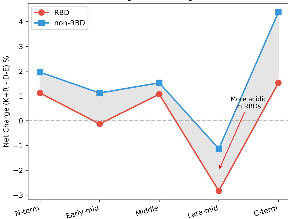
Net Charge Profile Along Domain
