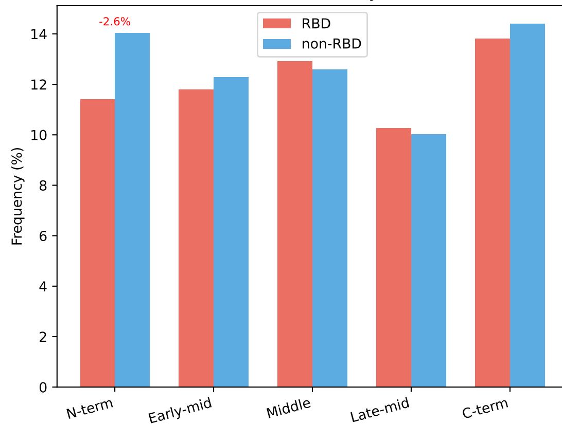
Basic (K+R) Residues by Position
