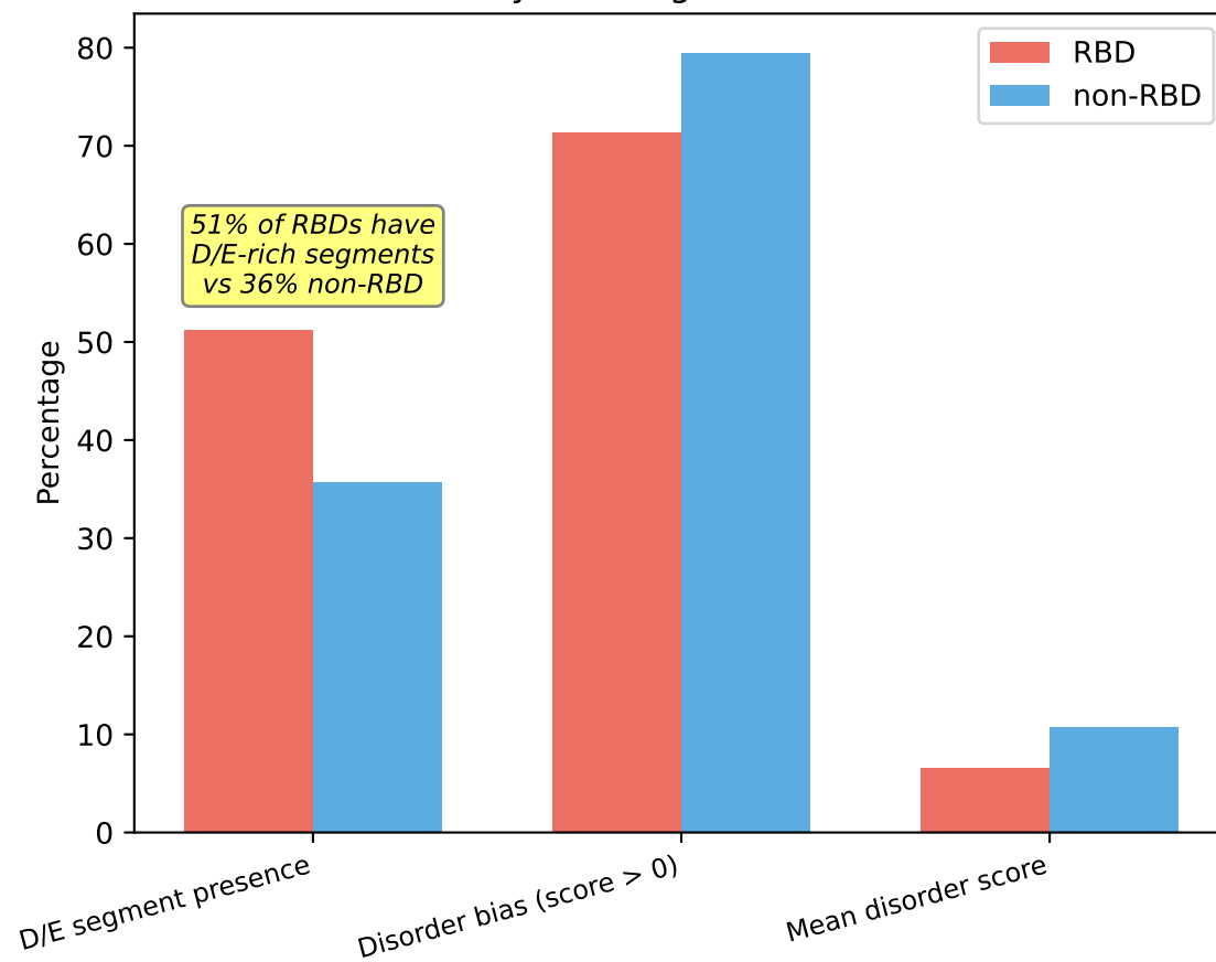
Summary: D/E Segments & Disorder
