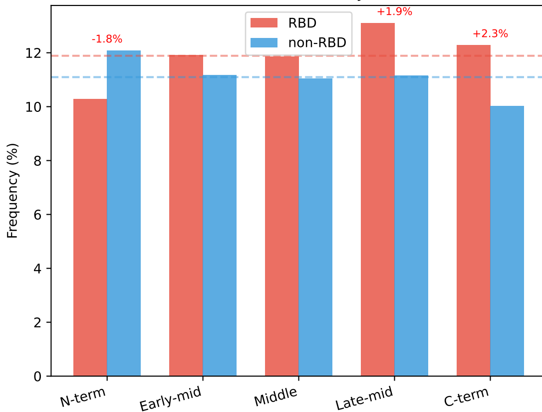
Acidic (D+E) Residues by Position
