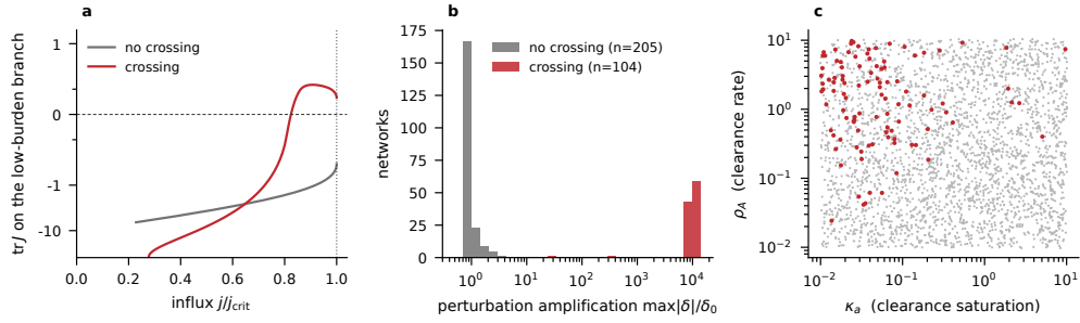
Fig. 4 The fold is not always the first loss of stability. (a) \operatorname{tr} J along the low-burden branch against j/j_{\text{crit}} , on a symmetric-log axis, for one crossing network and one non-crossing network. Both exemplars are chosen by rule rather than by inspection: the crossing case is the network nearest the median crossing position among those whose branch is resolved below 0.3 j_{\text{crit}} , and the non-crossing case is the network nearest the population median of \max(\operatorname{tr} J) . The crossing exemplar happens to be one of the 61 that do not recover, so its trace stays positive to the fold; a window network would return below zero before reaching it. (b) Amplification of a perturbation applied at each network's own \operatorname{tr} J maximum, integrating the full nonlinear system. Of the 108 crossing networks the 104 whose branch maximum is the fold were integrated: all grow by more than tenfold and 102 leave the linear neighbourhood, at a median amplification of 9851; the 205 non-crossing controls give 0 escapes and a median of 1.00. The distributions do not overlap, and this panel shares no failure mode with the branch computation in (a). It does not, however, separate a stable limit cycle from divergence — escape is a ten-thousandfold amplification and both produce it — which is what the Lyapunov classification in the text is for. (c) Where the crossing networks sit in the sampled (\kappa_a, \rho_A) plane. Relative to the rest they have \rho_A 7.5\times higher and \kappa_a 11.7\times lower: clearance that is fast and sharply saturating.
