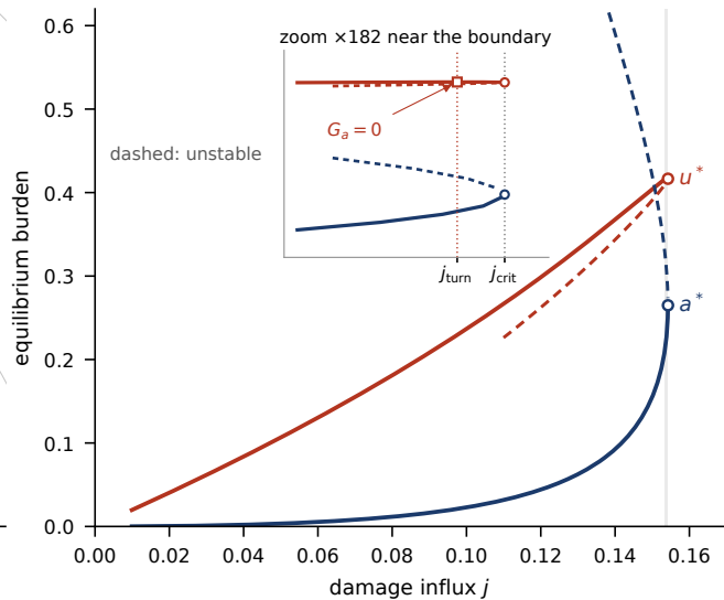
(b) two singularities, in order
