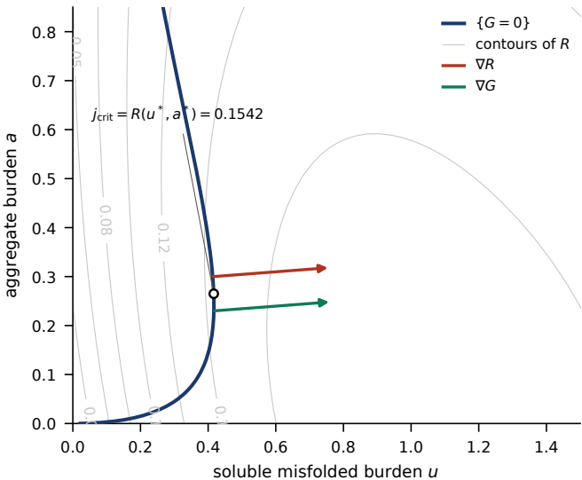
(a) the gradients align at the fold
