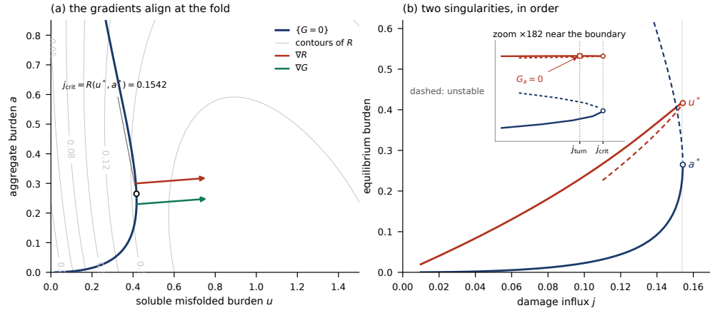
Fig. 1 The fold as a constrained critical point. (a) Phase plane at the base parameter point. The aggregate nullcline \{G = 0\} (dark) is a fixed curve; grey contours are total removal R . At the solved fold (u^*, a^*) = (0.4166, 0.2650) the gradients \nabla R and \nabla G point the same way, which is the Lagrange condition of Theorem 1; they are drawn from offset origins because, being parallel, a common origin hides one behind the other. The sine of the angle between them is 3.5 \times 10^{-10} . The critical influx is the removal flux evaluated there, j_{crit} = R(u^*, a^*) = 0.1542 . (b) Both equilibrium coordinates against influx, traced along the same curve. Cramer's rule on the two columns gives du^*/dj = -G_a/\det J and da^*/dj = G_u/\det J , so the branch carries two distinct, ordered singularities. At j_{turn} = 0.15409 the soluble pool has a HORIZONTAL tangent, where G_a = 0 ; this is a regular point of the branch, since \det J = R_a \cdot G_u = 2.027 \times 10^{-3} there rather than zero, and it lies on the stable branch at j_{turn}/j_{crit} = 0.9990 . At j_{crit} both coordinates have a VERTICAL tangent, which is \det J = 0 . The inset is a \times 182 zoom on the same computed data, not a schematic. The aggregate coordinate has no horizontal tangent anywhere: G_u > 0 at all 305 traced points (minimum 2.08 \times 10^{-3} ), and in 40 draws from the parameter box no point with G_u < 0 was found, for the reason given in Section 3.1.
