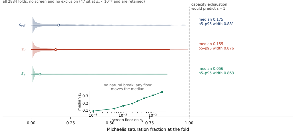
Fig. 3 Saturation of the clearance machinery at the fold, over all 2884 kinetic-box folds with none excluded. The distributions are evaluated at the recorded continuation states, where Section 6’s table is evaluated at re-solved states satisfying \{G = 0, \det J = 0\} ; the two populations differ by the 117 networks that do not re-solve and the medians differ in the third decimal, so the medians are quoted in the table only. The p5–p95 widths here are 0.881, 0.876 and 0.863. The point the figure carries is the width, not the centre: the spans are wide enough that a single measurement discriminates weakly against the capacity-exhaustion alternative. Inset: median s_a against an imposed lower screening floor, from 0.090 at a floor of 10^{-4} to 0.355 at 2 \times 10^{-2} . The distribution runs smoothly across five decades with no gap, so any floor is a free parameter that moves a load-bearing median by a factor of four. No floor is applied anywhere in this paper.
