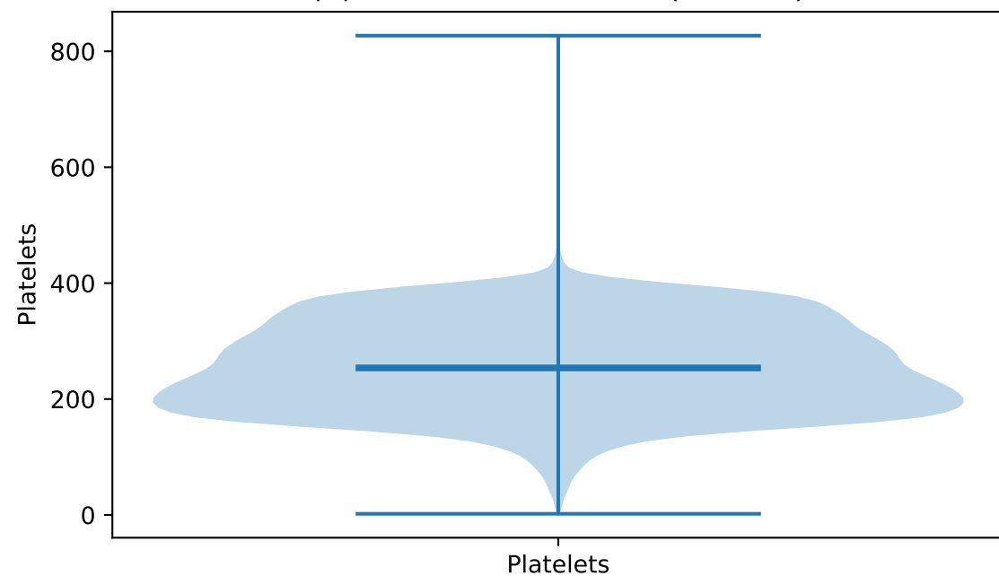
(C) Platelets distribution (n=5901)
