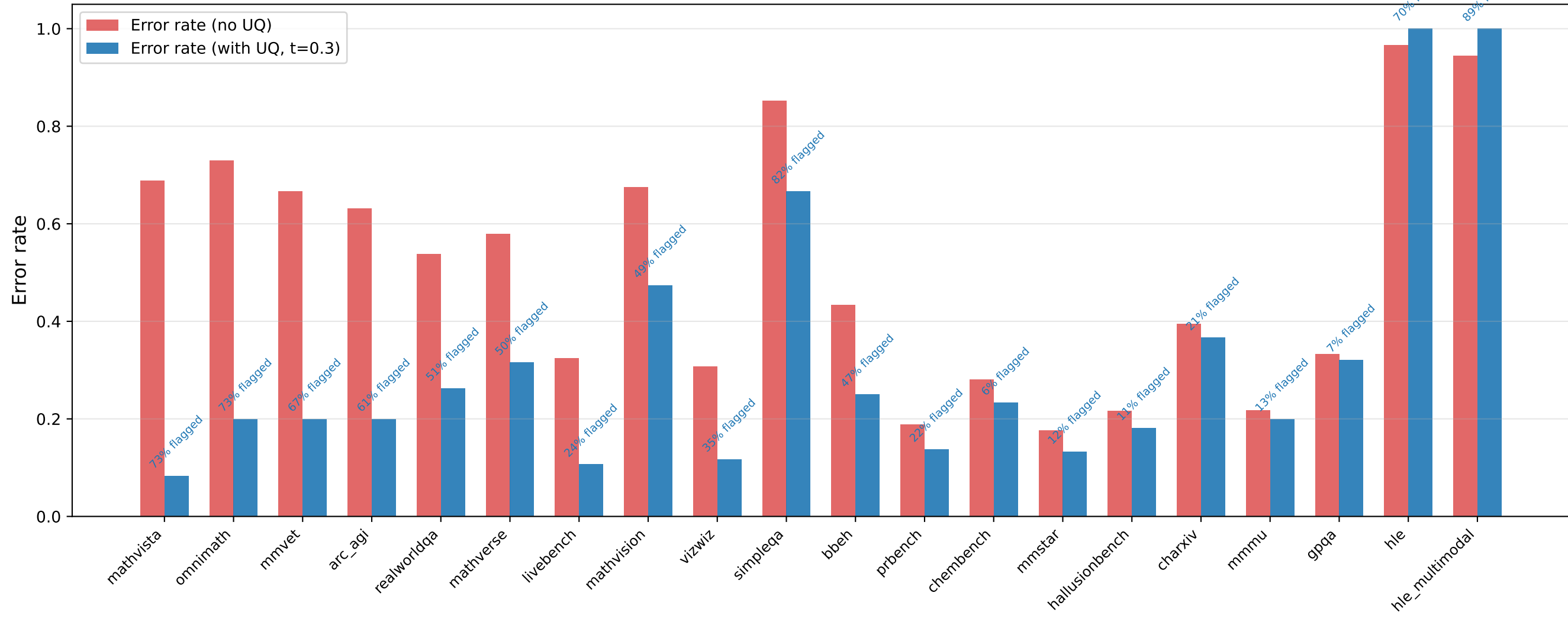
UC-E: Error Reduction by Benchmark — GPT-5-mini (flag if p_correct < 0.3)
