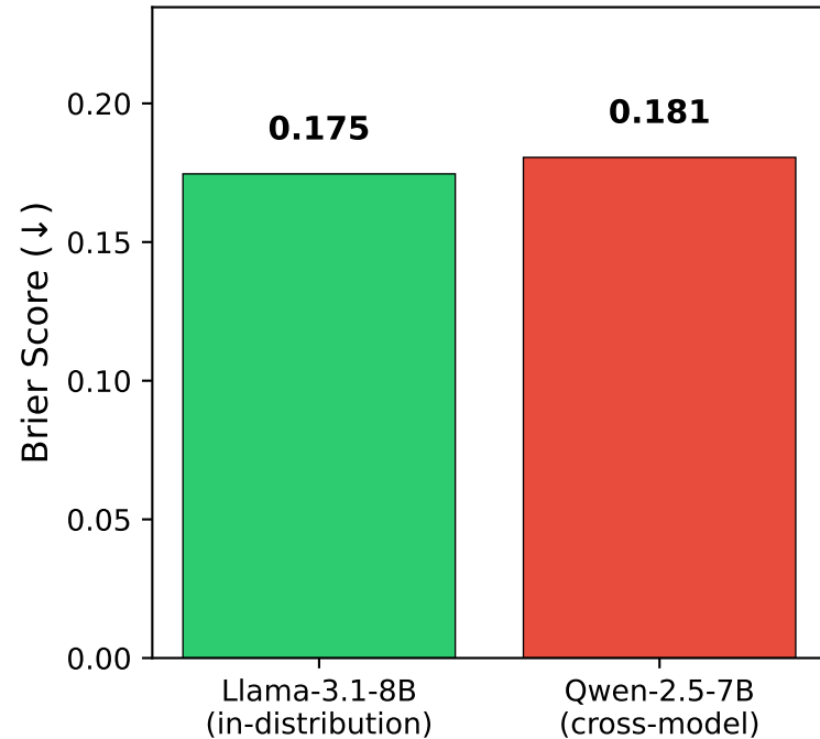
Overall Quality
