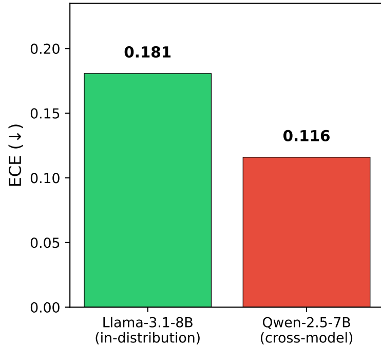
Calibration Error
