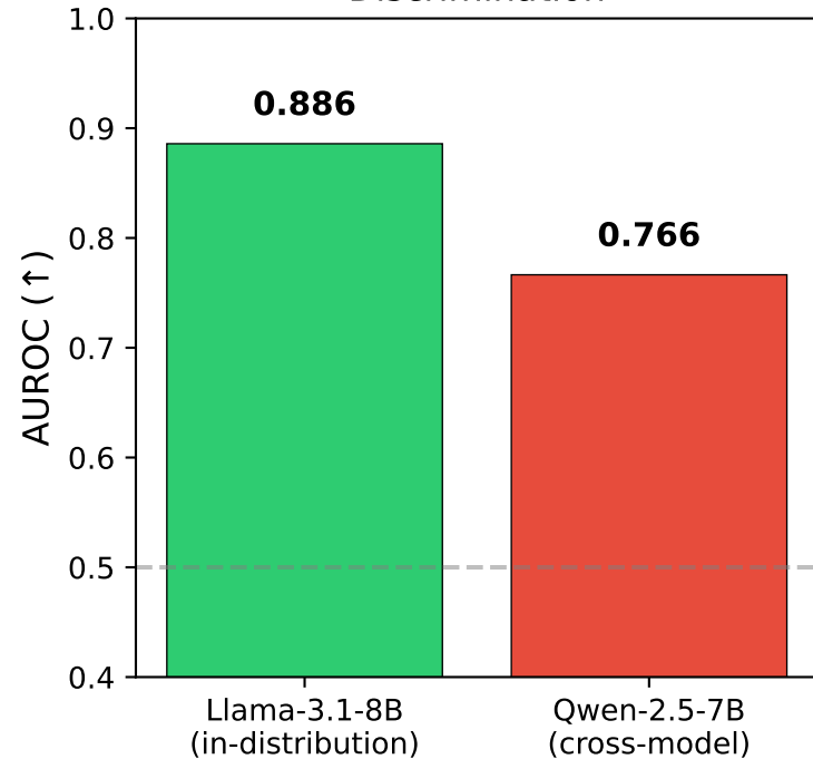
Discrimination
