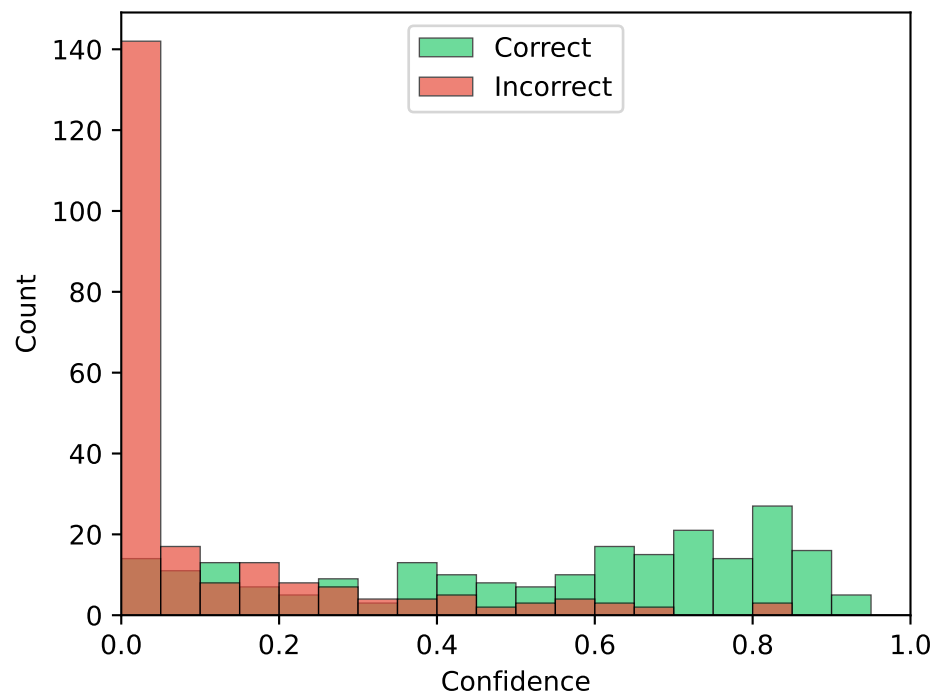
Zero-shot
