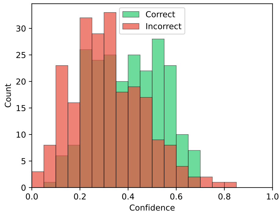
Zero-shot
