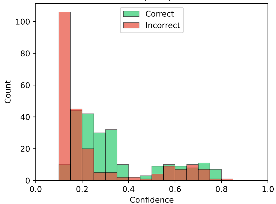
Perplexity
