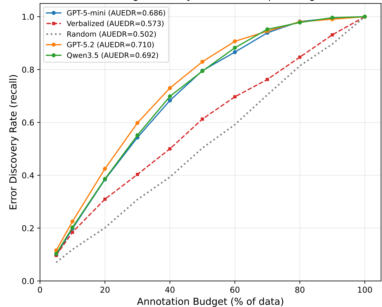
Labeling Efficiency: Errors Found per Budget
