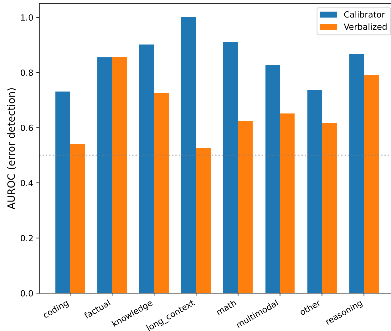
Per-Domain Error Detection — GPT-5-mini
