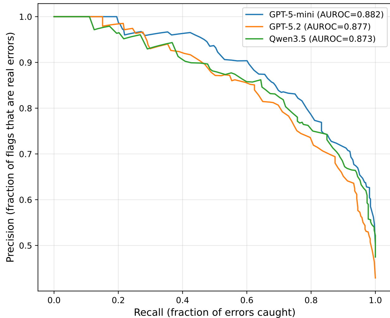
Error Detection: Precision-Recall
